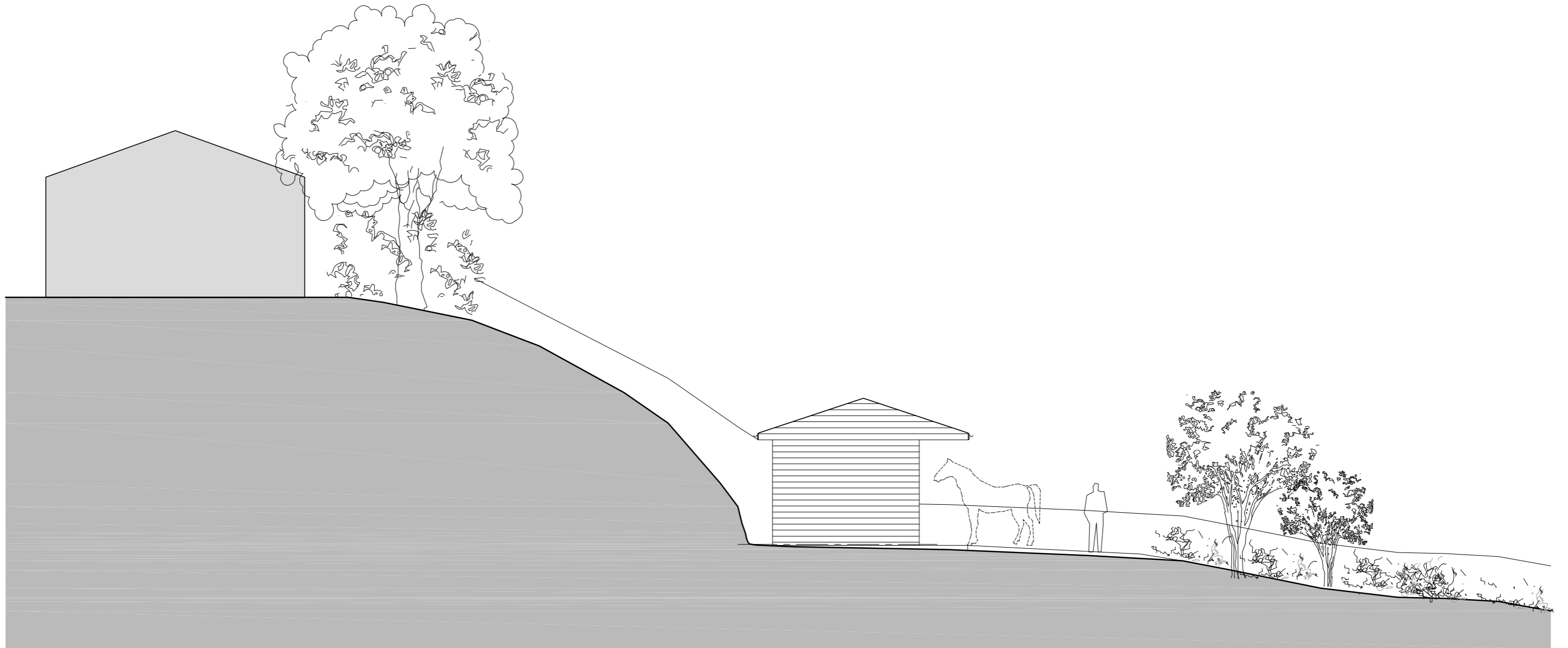
site cross section
