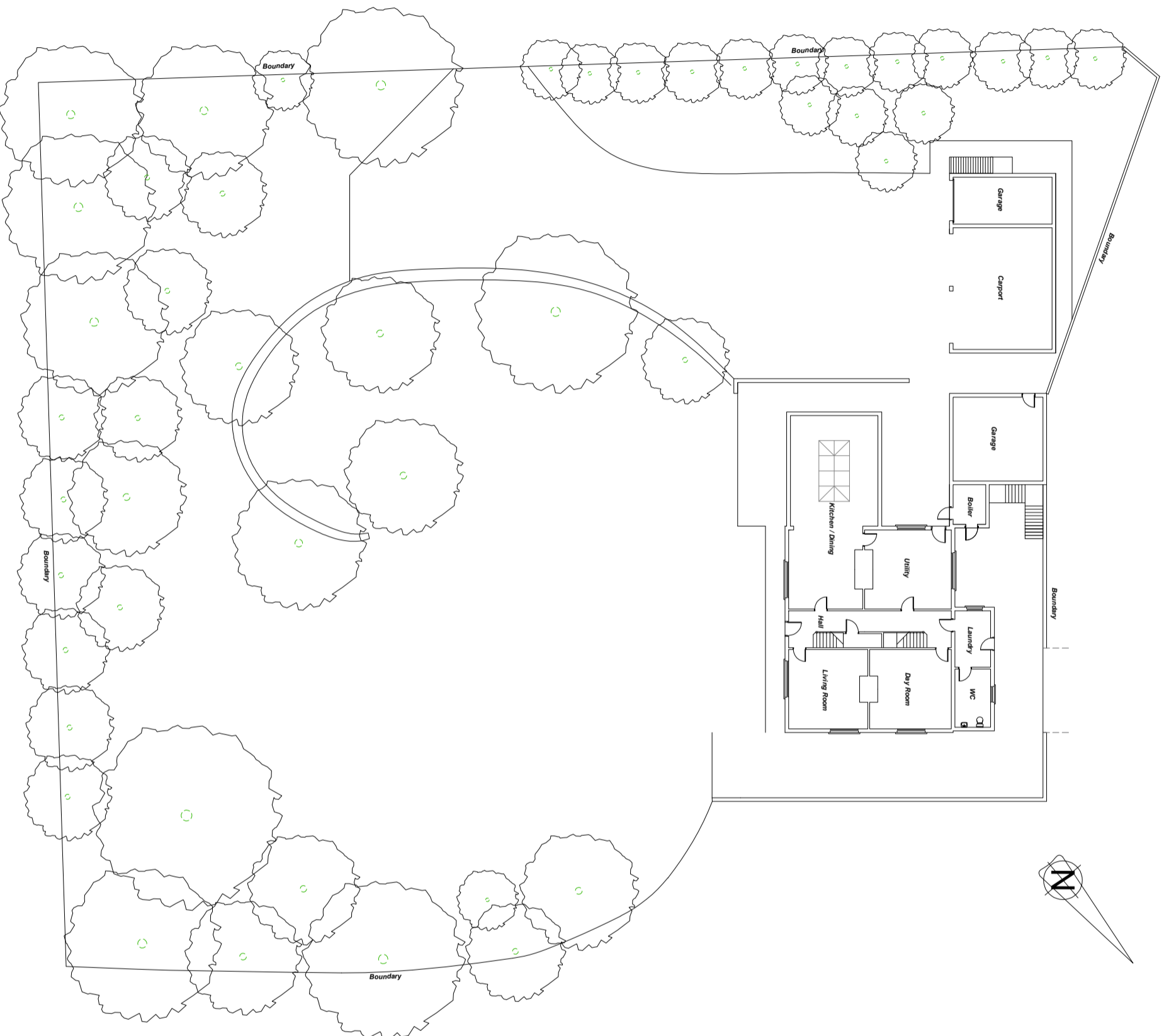
Site Plan as Proposed Scale 1:300
