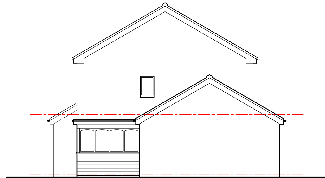
Side-01 elevation 1:100
