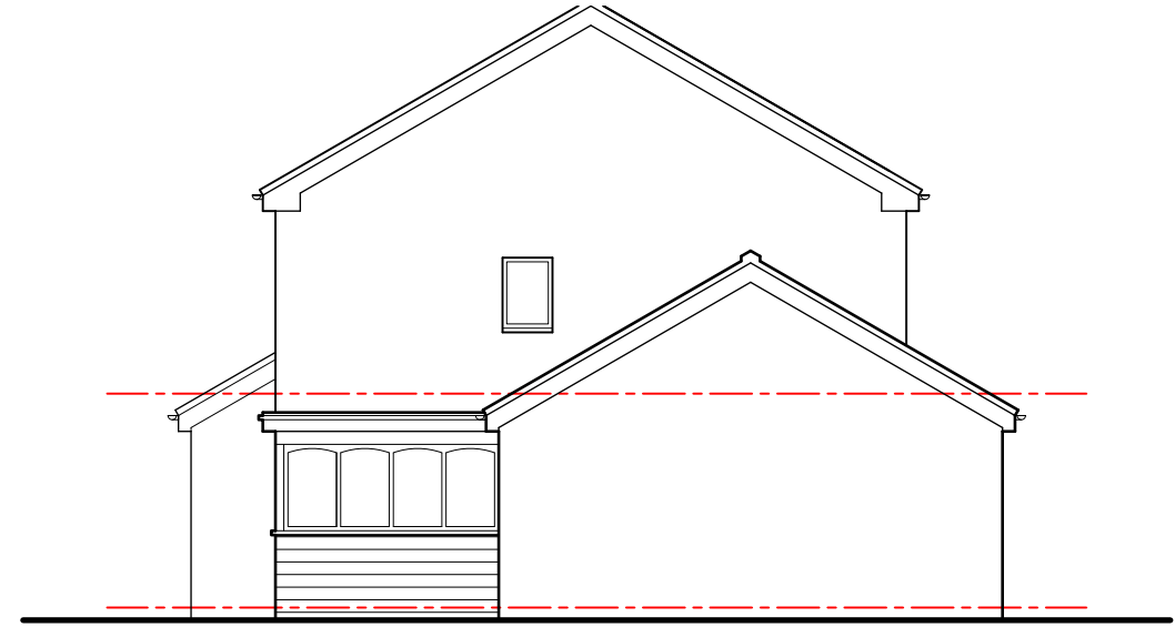
Side-01 elevation 1:100
