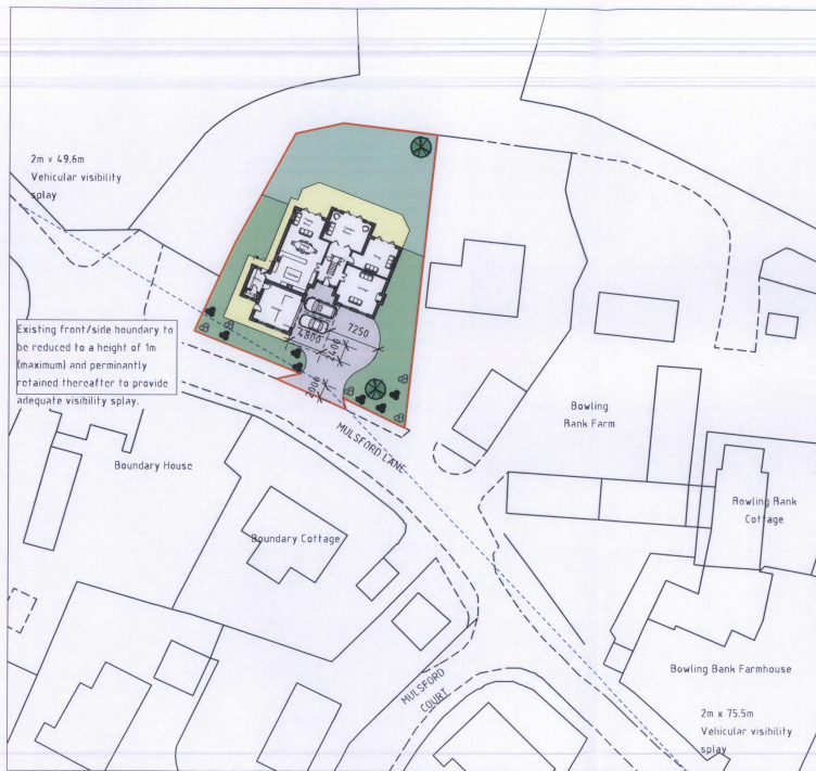
Highways Plan 1:500
