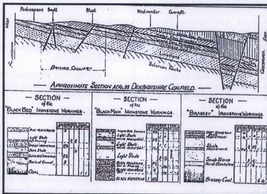
Cross Section through Brymbo Colliery showing fault and Main Ironstone horizons
