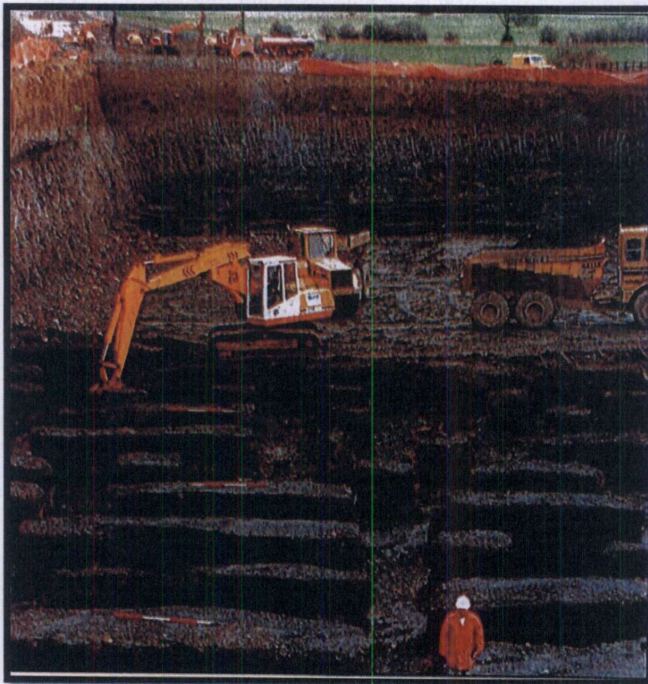
Example of pillar and stall workings exposed in an opencast
