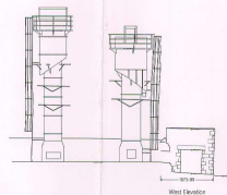
West Elevation
