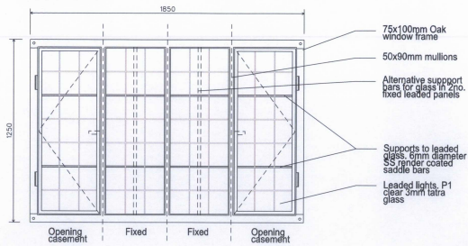
Window type.01 Windows WG02, WG03, WG04, WF01, WF02, WF03
