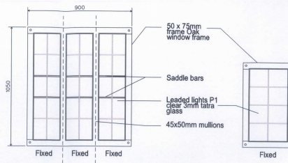
Window type.03 Window WF04
