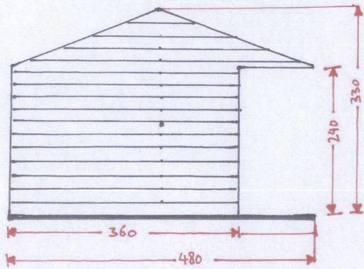
LEFT ELEVATION SCALE 1:50
