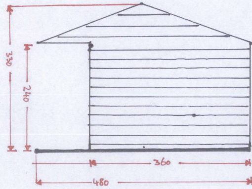
RIGHT ELEVATION SCALE 1:50
