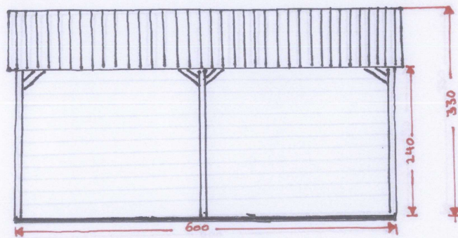
FRONT ELEVATION SCALE 1:50
