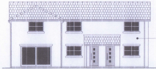
PROPOSED ELEVATION (North West)
