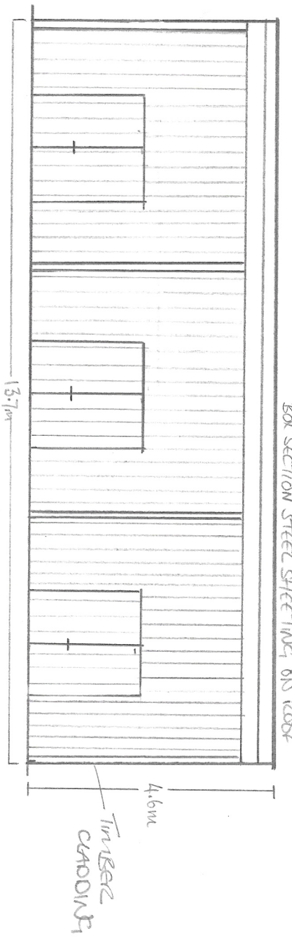
FRONT ELEVATION -
