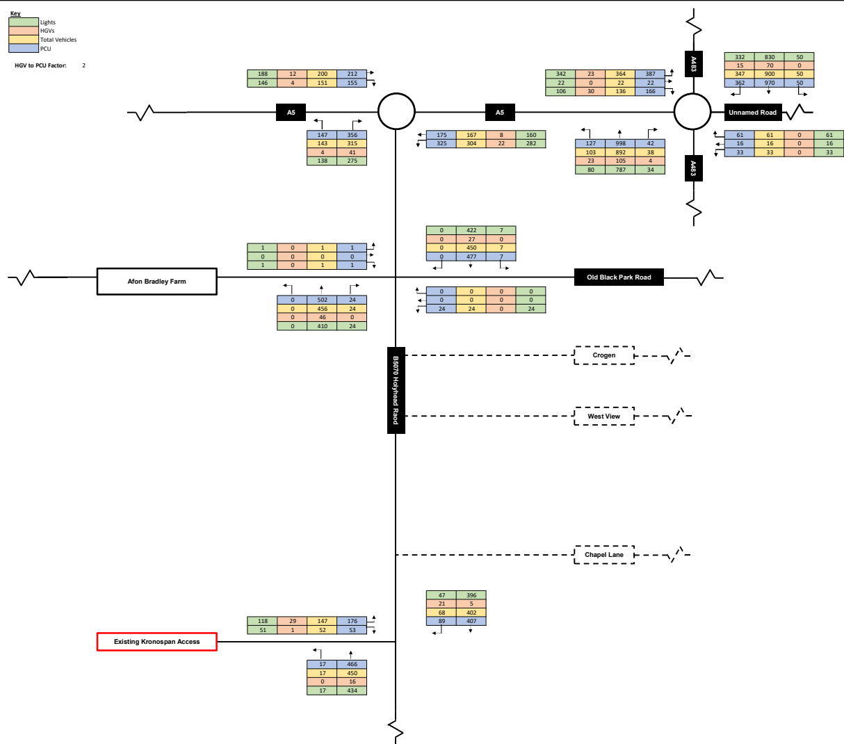
Figure: 10 Project Name: Kronospan Northern Infrastructure Project Number: 3162-01 Description: 2031 'Do Nothing' Without Development Scenario Period: PM (5:00pm - 6:00pm)
