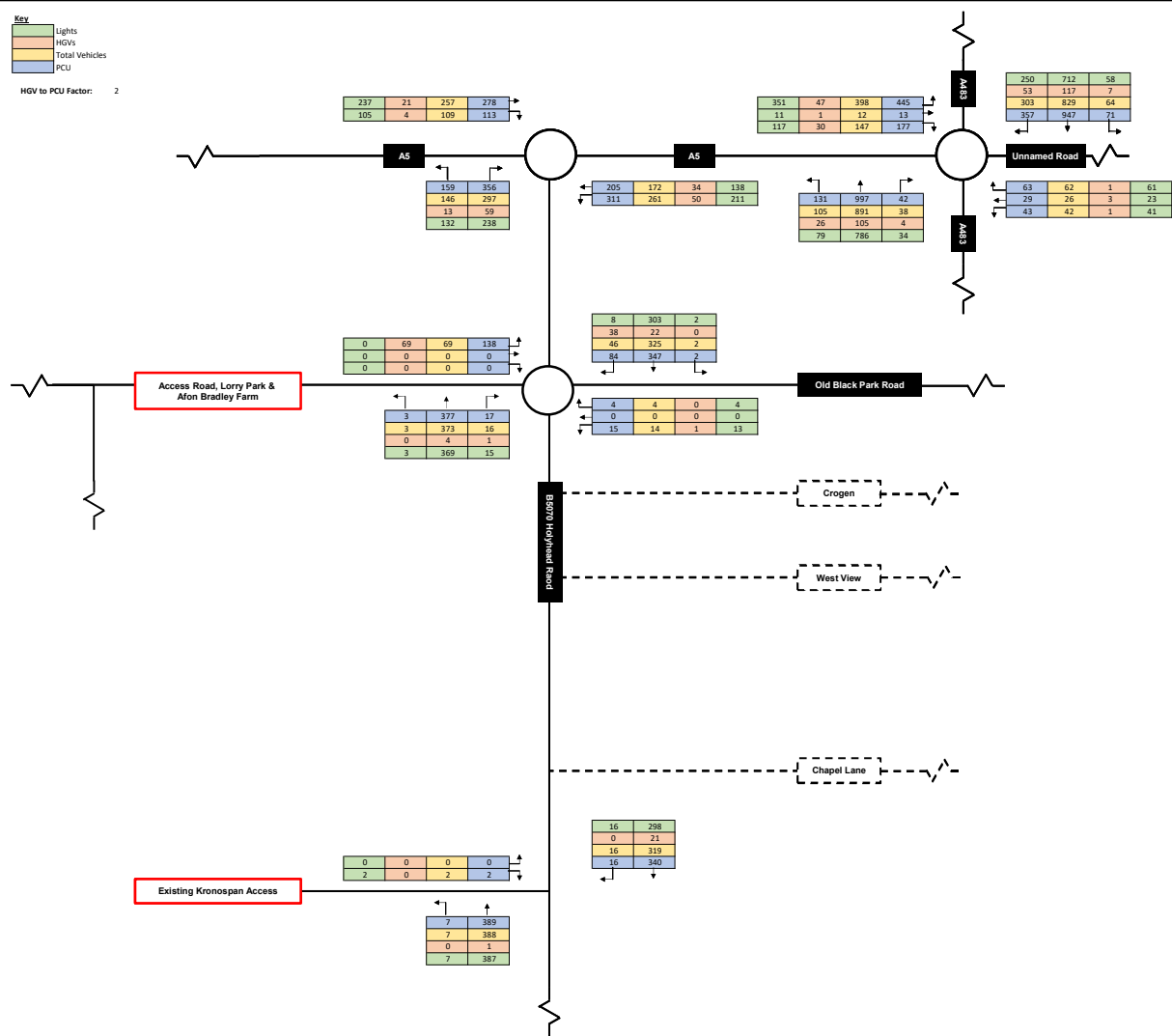
Figure: 13 Project Name: Sandown Quarry Project Number: 3162-01 Description: 2026 'Do Something' With Development Scenario Period: AM (8:00am - 9:00am)
