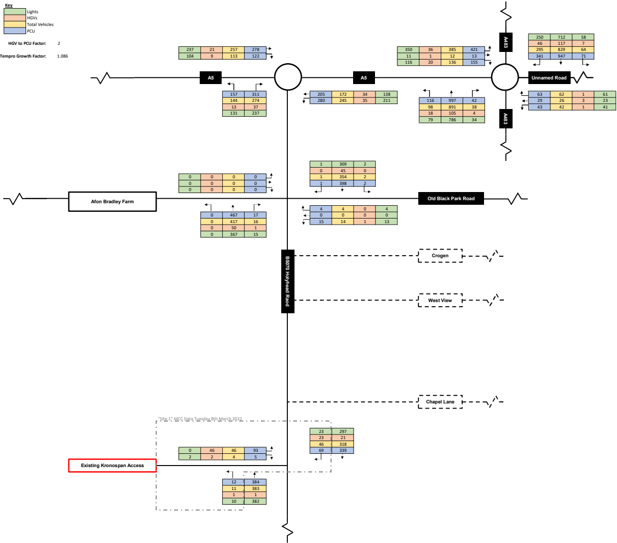
Figure: 5 Project Name: Kronospan Northern Infrastructure Project Number: 3162-01 Description: 2031 Factored Baseline Period: AM (8:00am - 9:00am)
