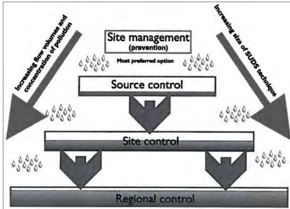
Figure 6-2 SuDS Management Train (from CIRIA C753)
