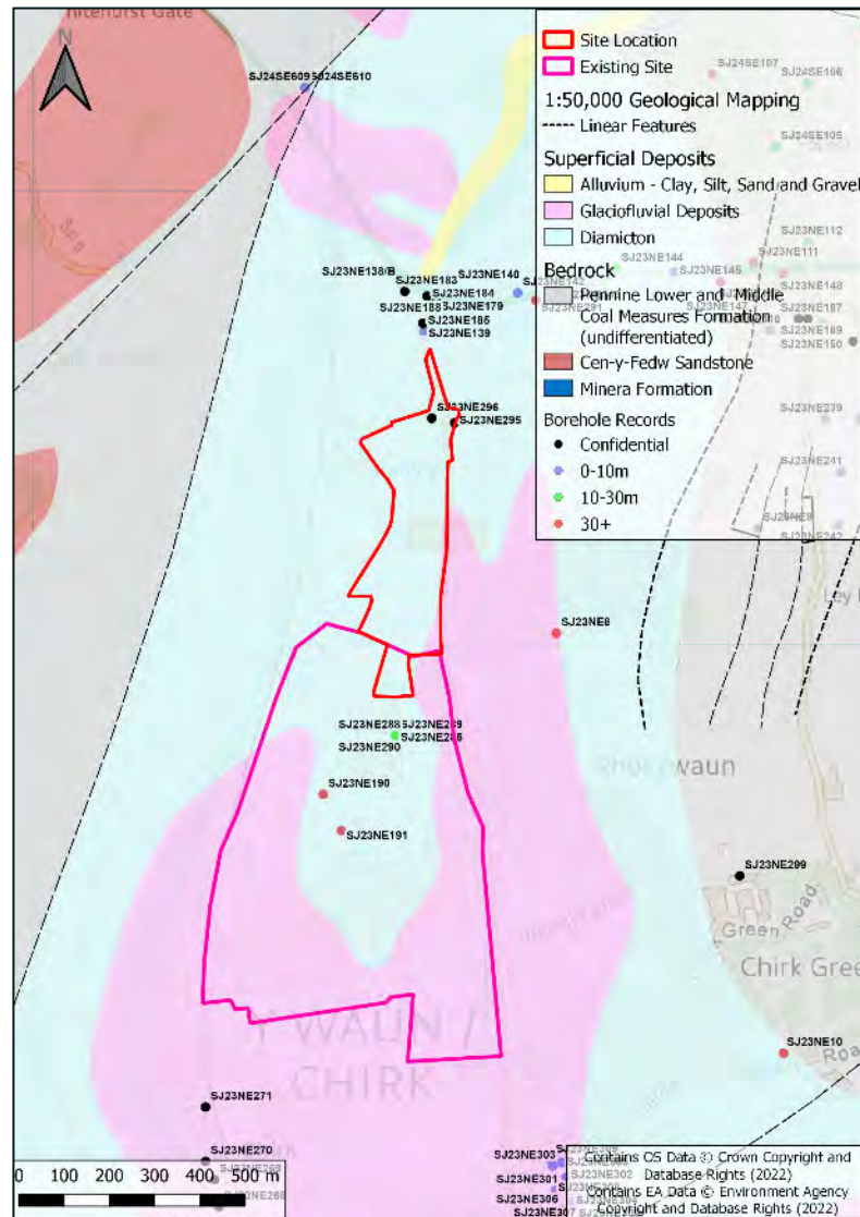
Figure 2-3 1:50,000 Mapped Geology
