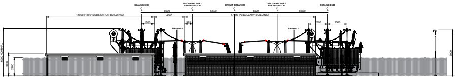
ELEVATION B - B (SCALE 1:500)
