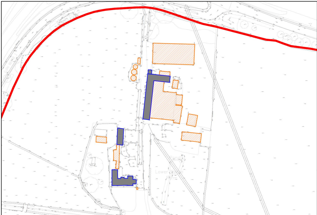
Figure 7: Demolitions at Lower Berse Farmhouse (hatched orange)
