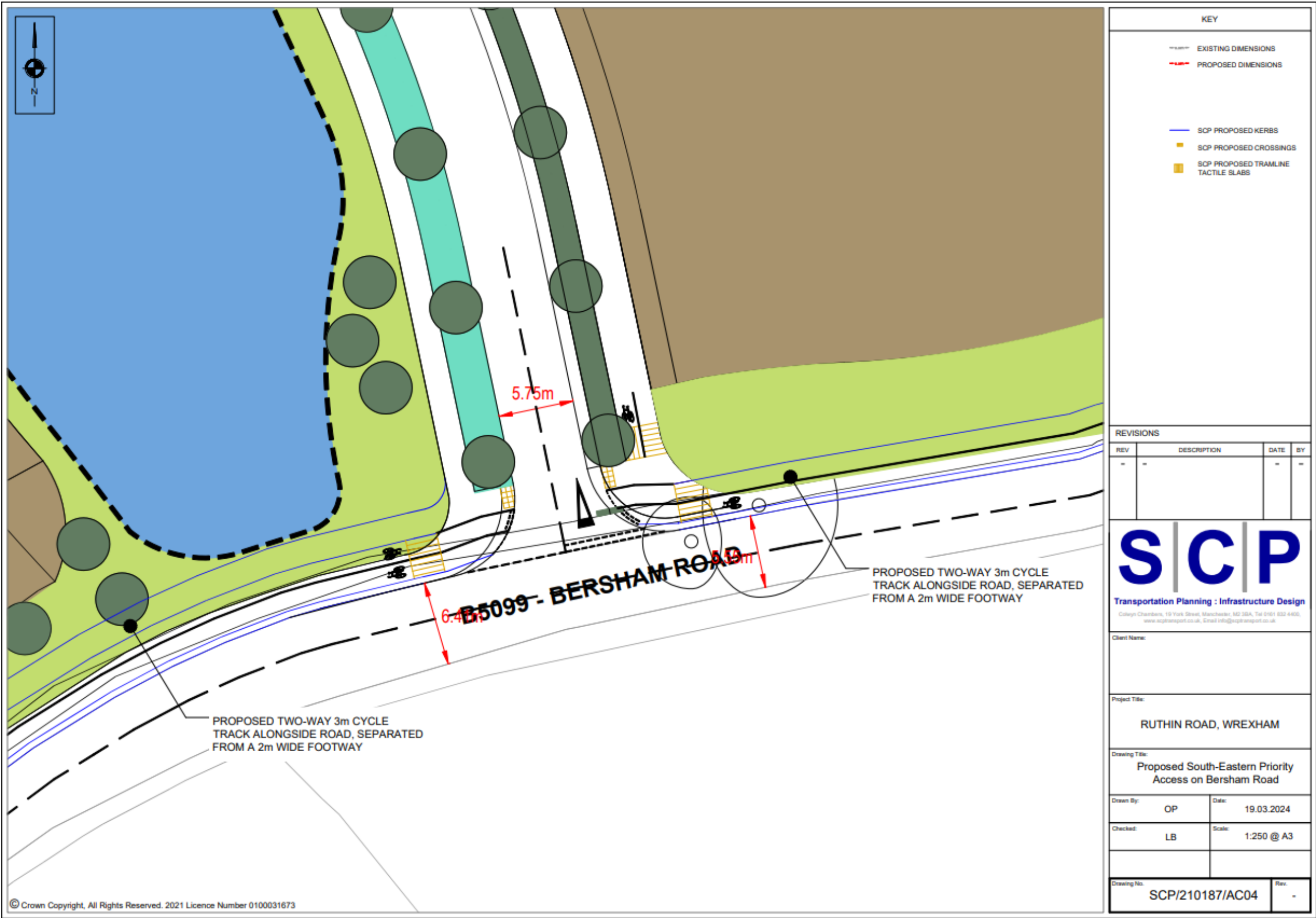
Figure A4: Proposed South-Eastern Priority Access on Bersham Road
