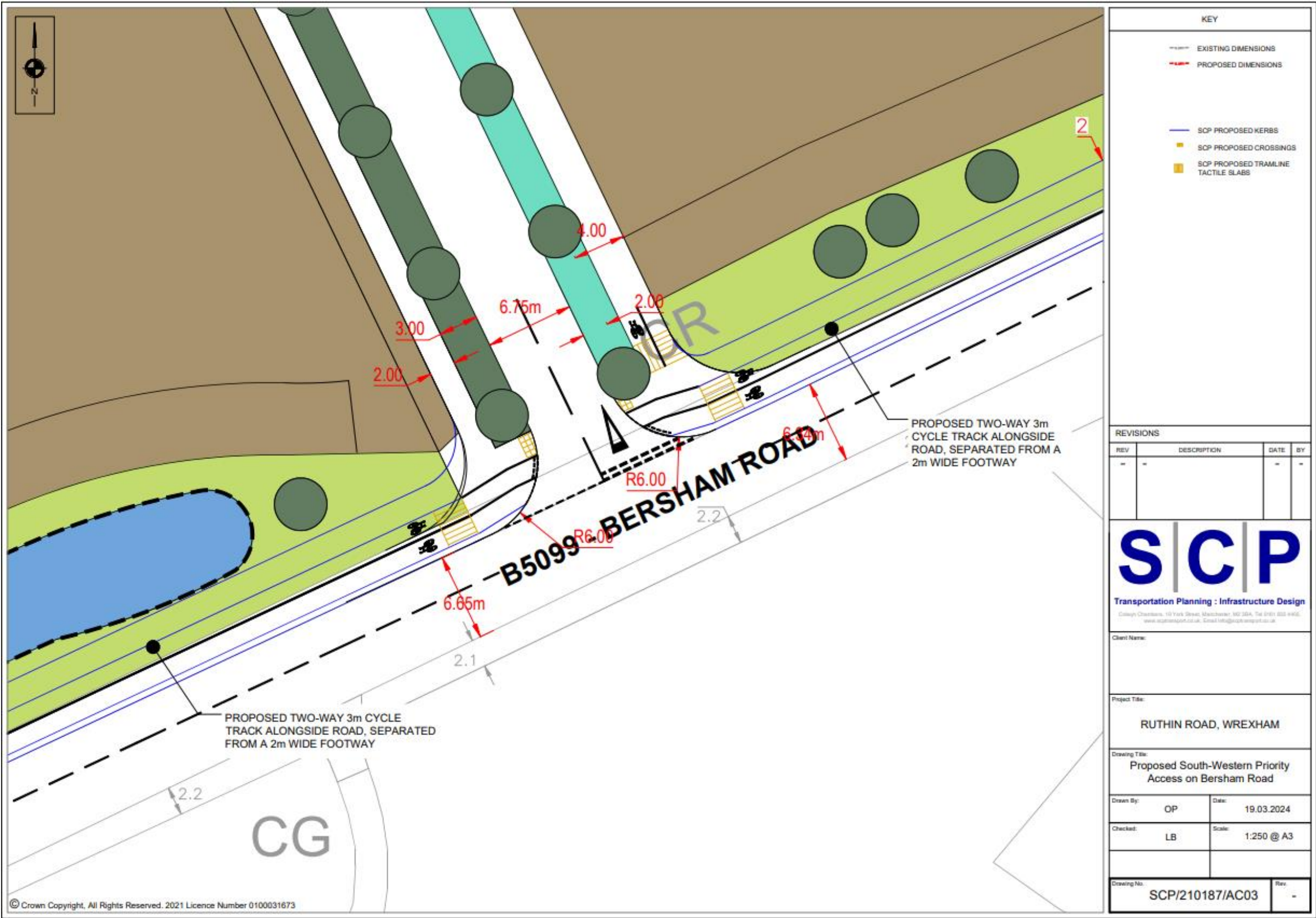
Figure A3: Proposed South-Western Priority Access on Bersham Road
