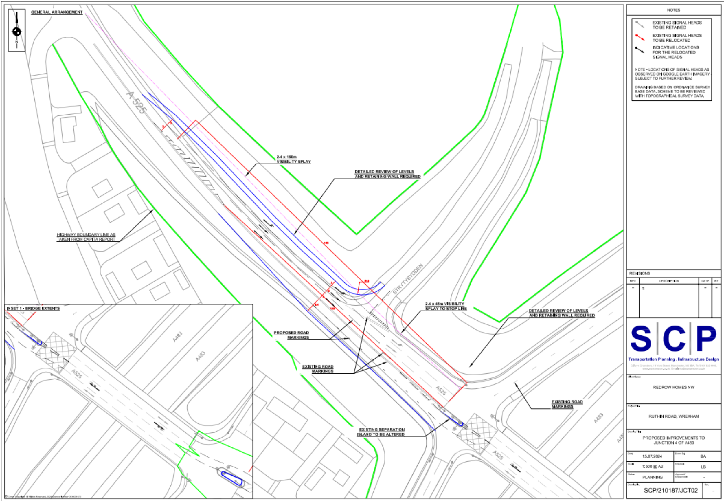
Figure A6: Proposed Junction Improvements at A483 Junction 4 – Western Portion of the Junction
