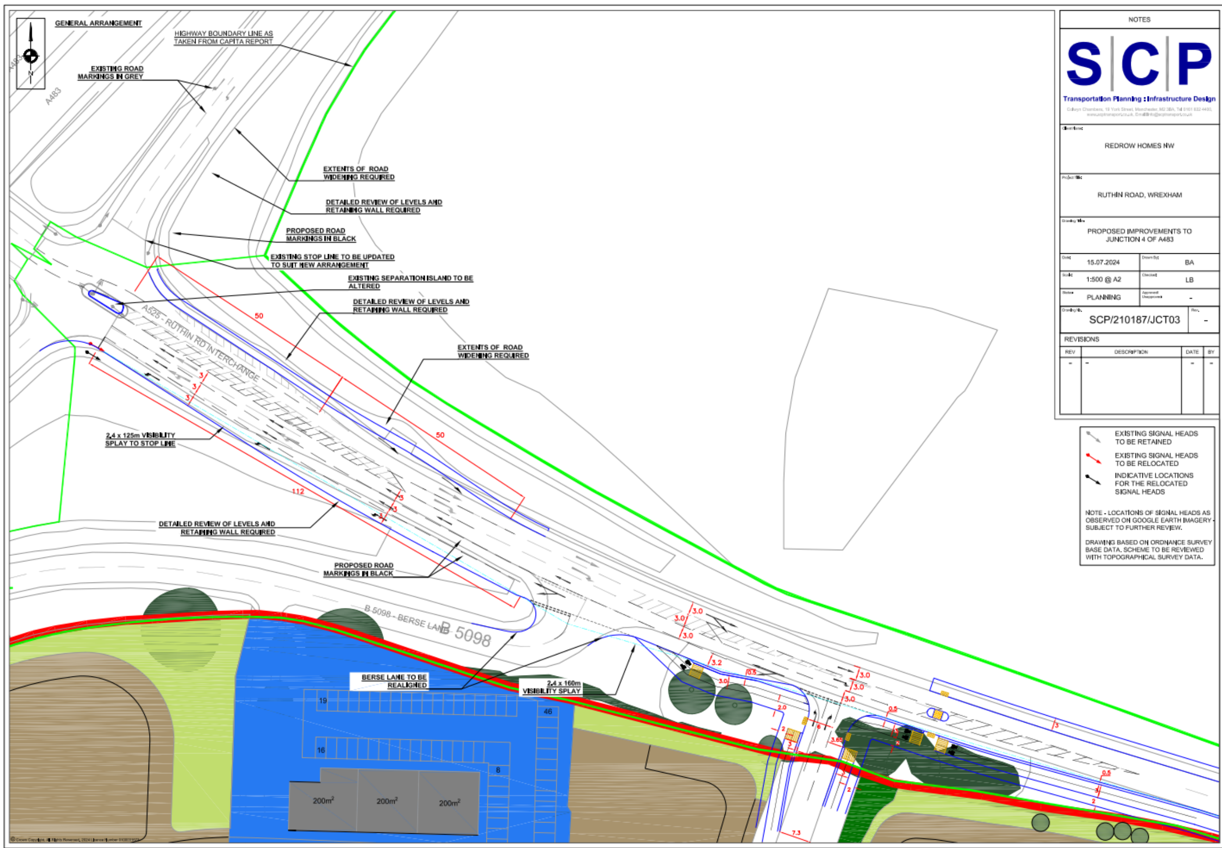
Figure A7: Proposed Junction Improvements at A483 Junction 4 – Eastern Portion of the Junction
