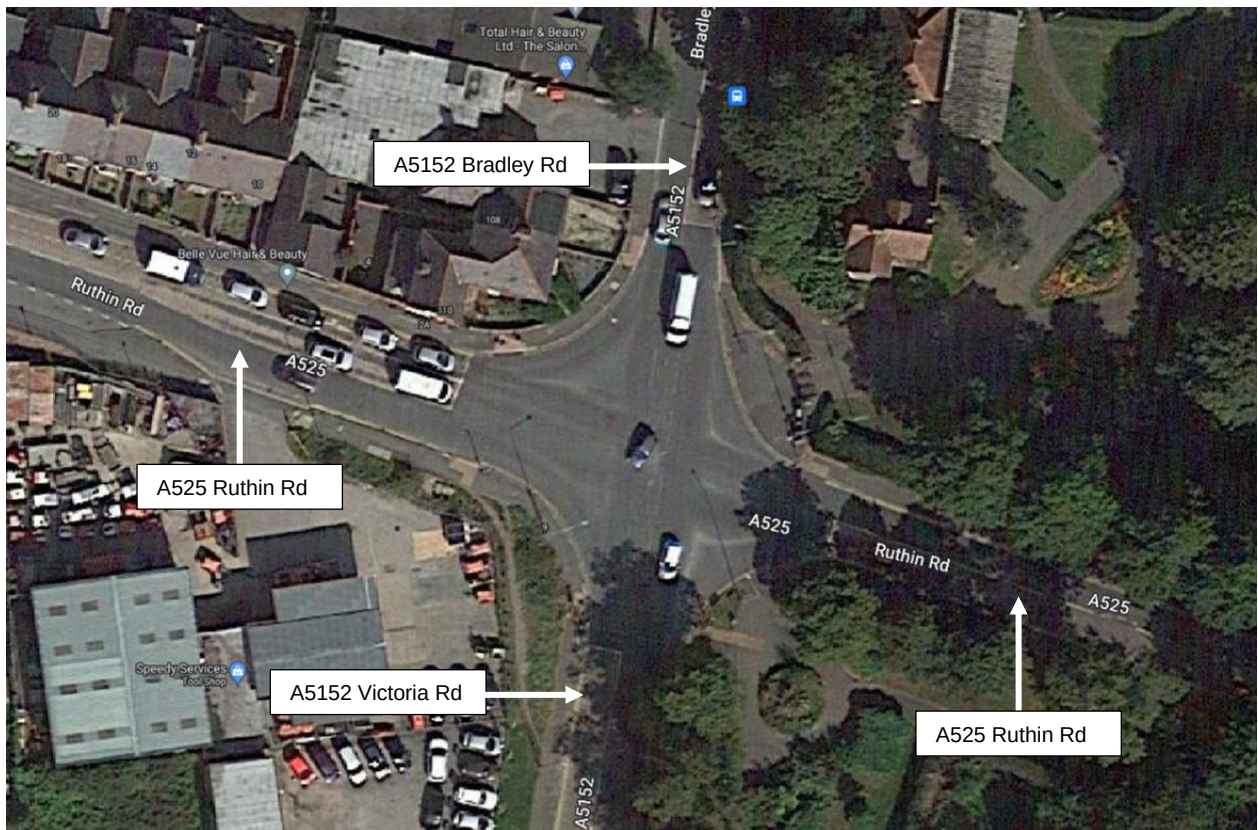
Figure 3.10 - A525 Ruthin Road / A5152 Signalised Crossroads
