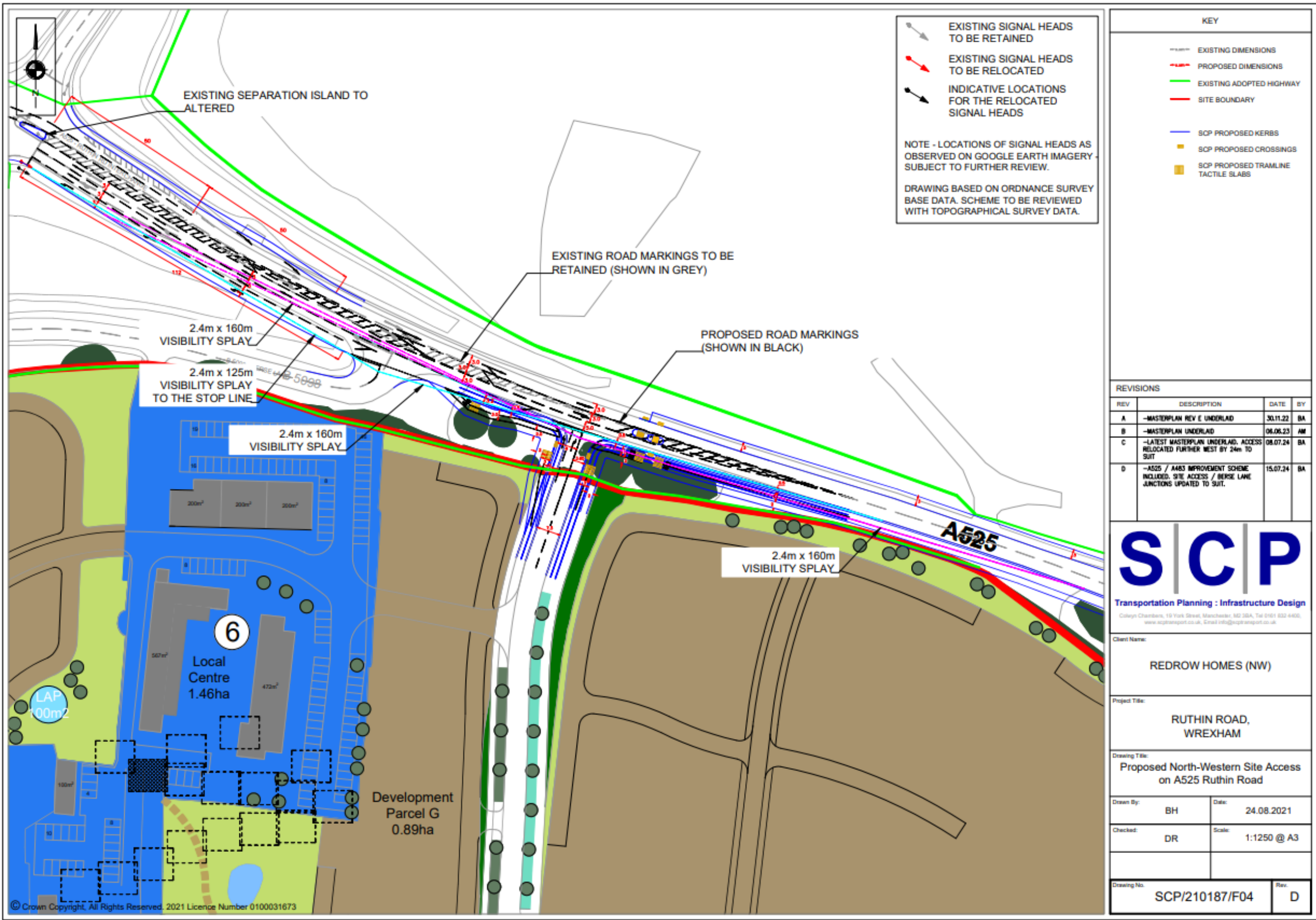
Figure A2: Proposed North-Western Site Access on A525 Ruthin Road
