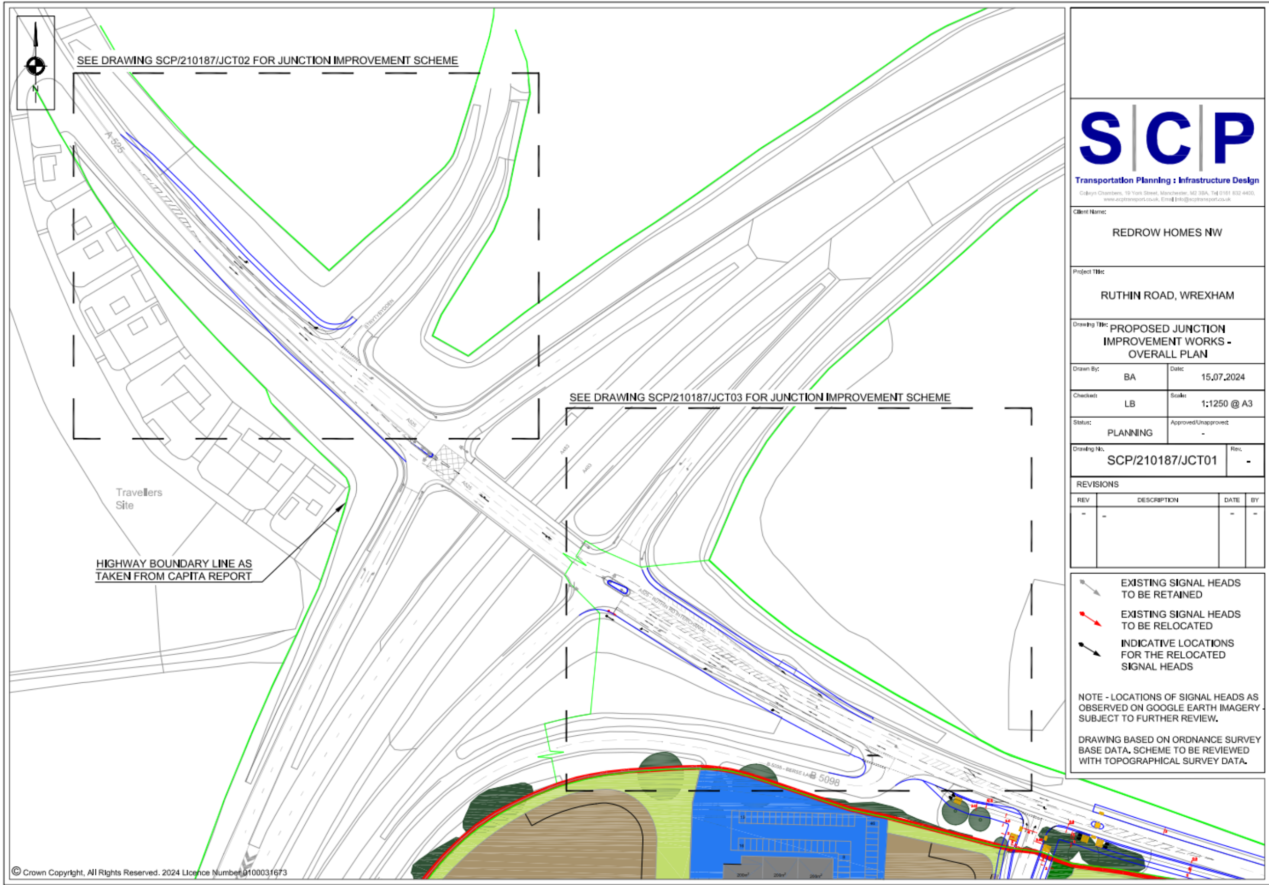
Figure A5: Proposed Junction Improvements at A483 Junction 4 - Overview
