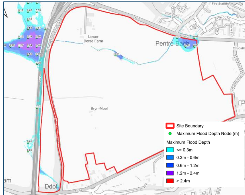
Figure 2 – Existing Scenario 1% AEP plus 45% CC Event – Flood Depths (m)
