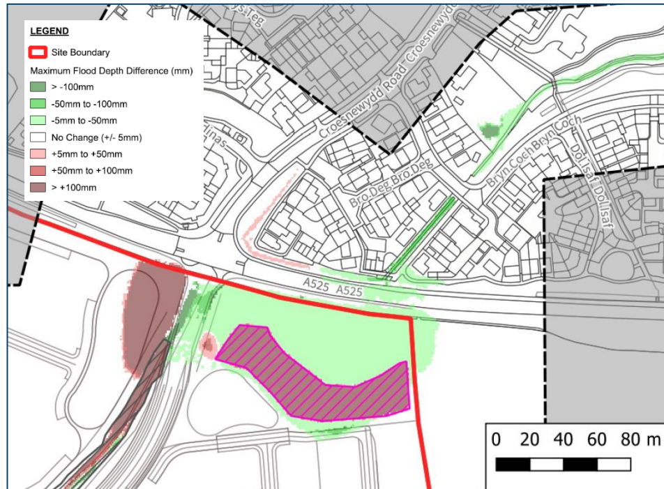
Figure 6 – 0.1% AEP plus 45% CC Depth Difference
