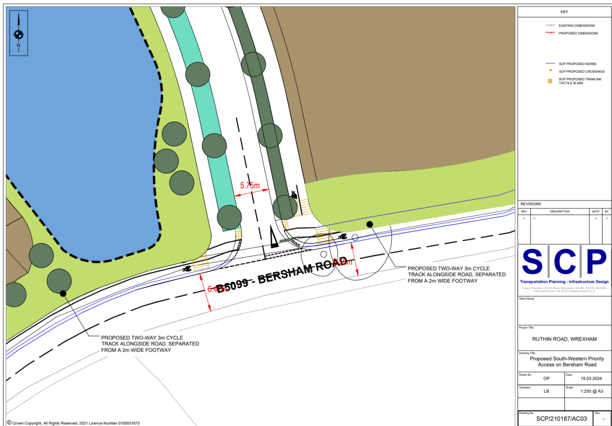
Figure 4.6: Bersham Road Access 1
