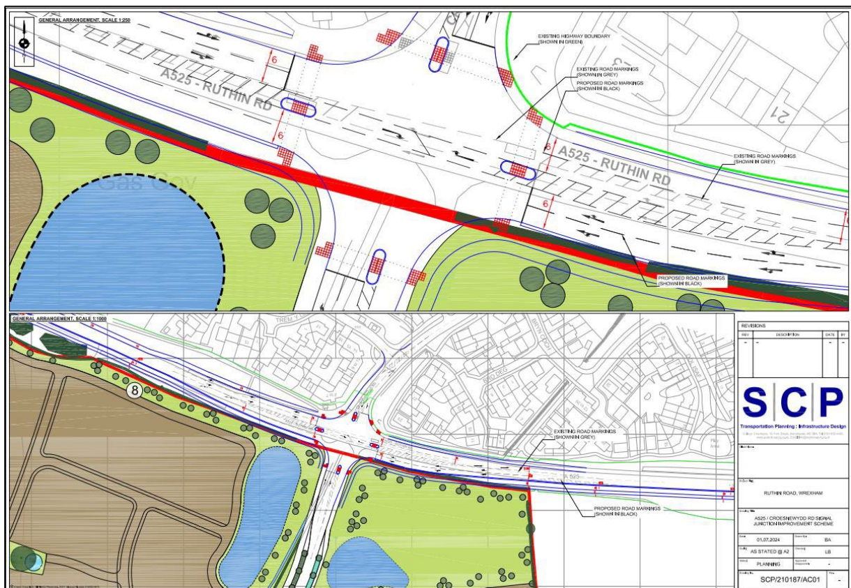
Figure 4.4: Ruthin Road Access 1
