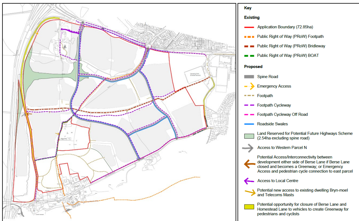
Figure 4.8: Access and Movement Parameters Plan
