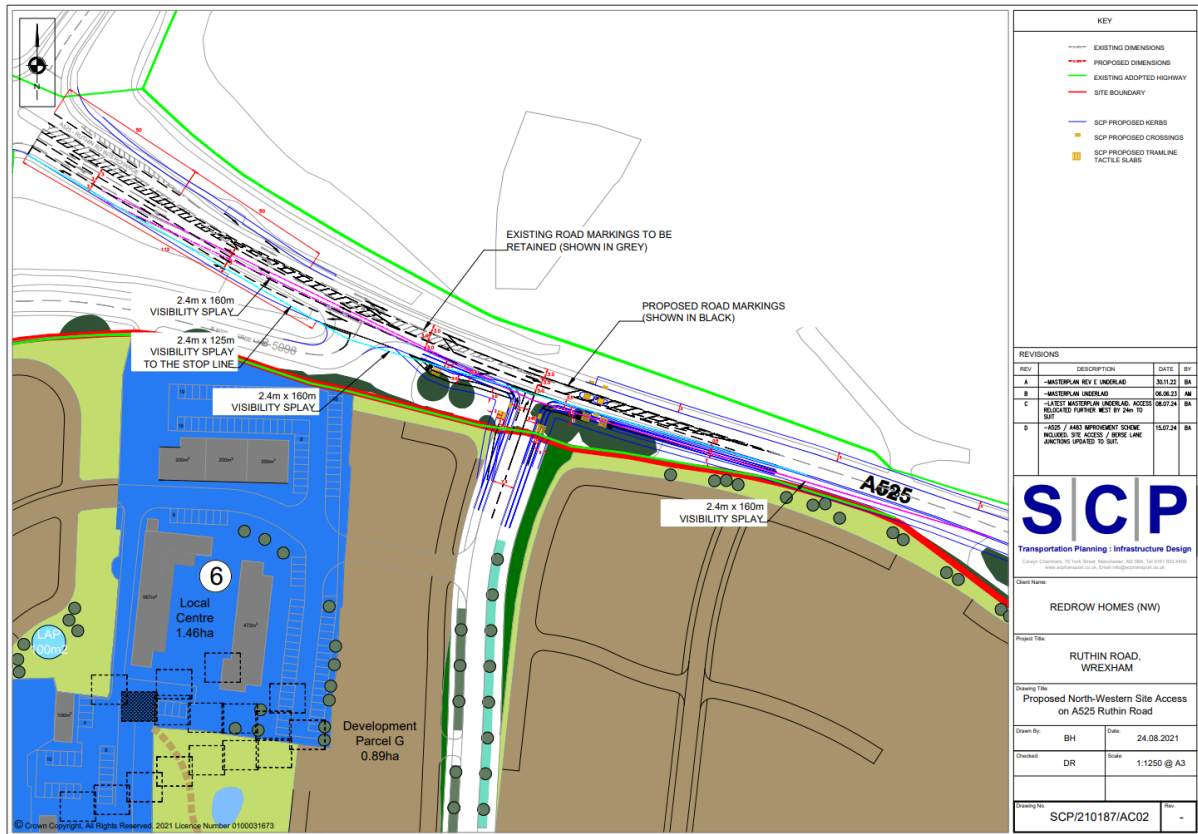
Figure 4.5: Ruthin Road Access 2
