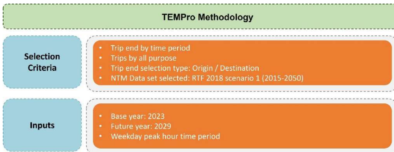
Figure 11: TEMPro Methodology
