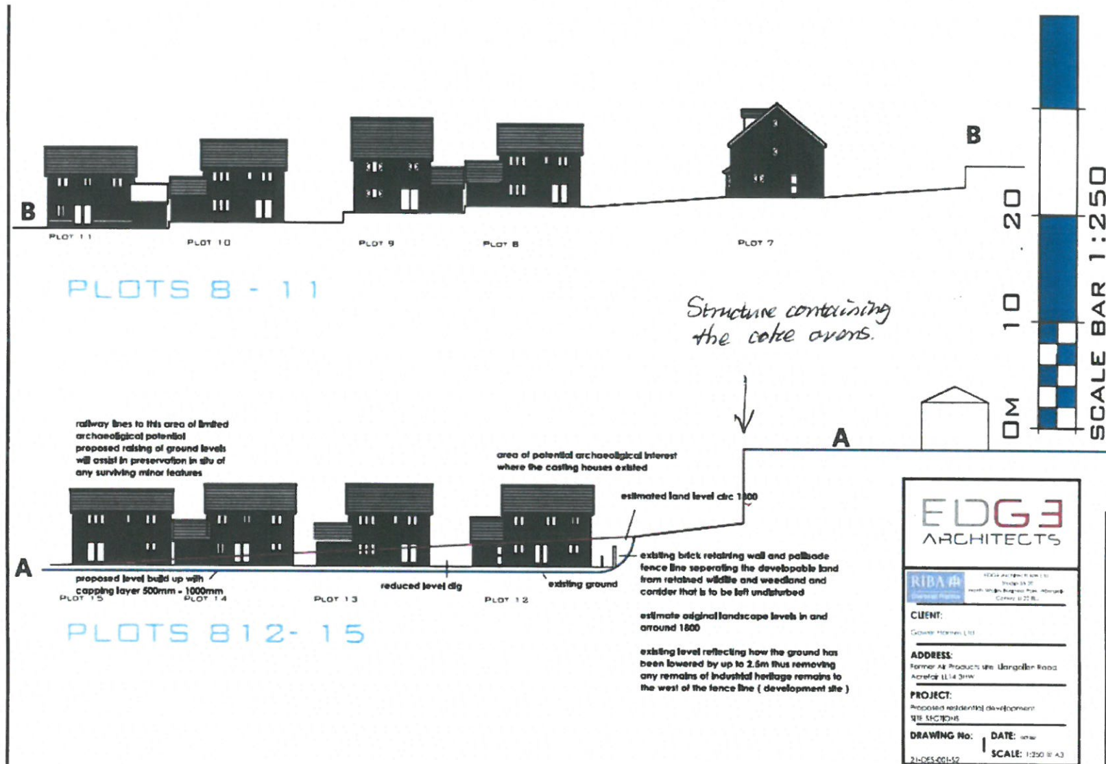
Figure 29 Site Cross Sections showing indicative ground levels and possible historic levels.
