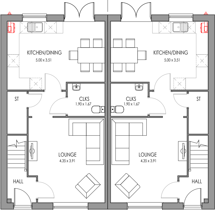
5P3B END AS GROUND FLOOR
