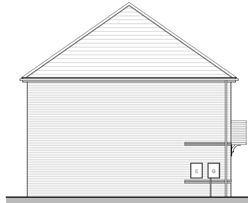
SIDE ELEVATION HB1
