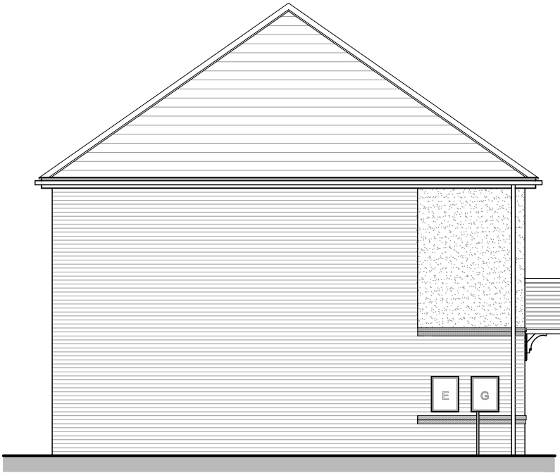
SIDE ELEVATION HR1
