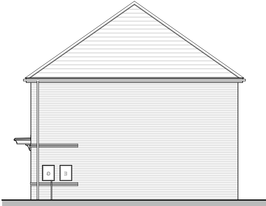
SIDE ELEVATION HB1
