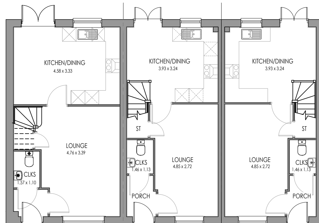
GROUND FLOOR
