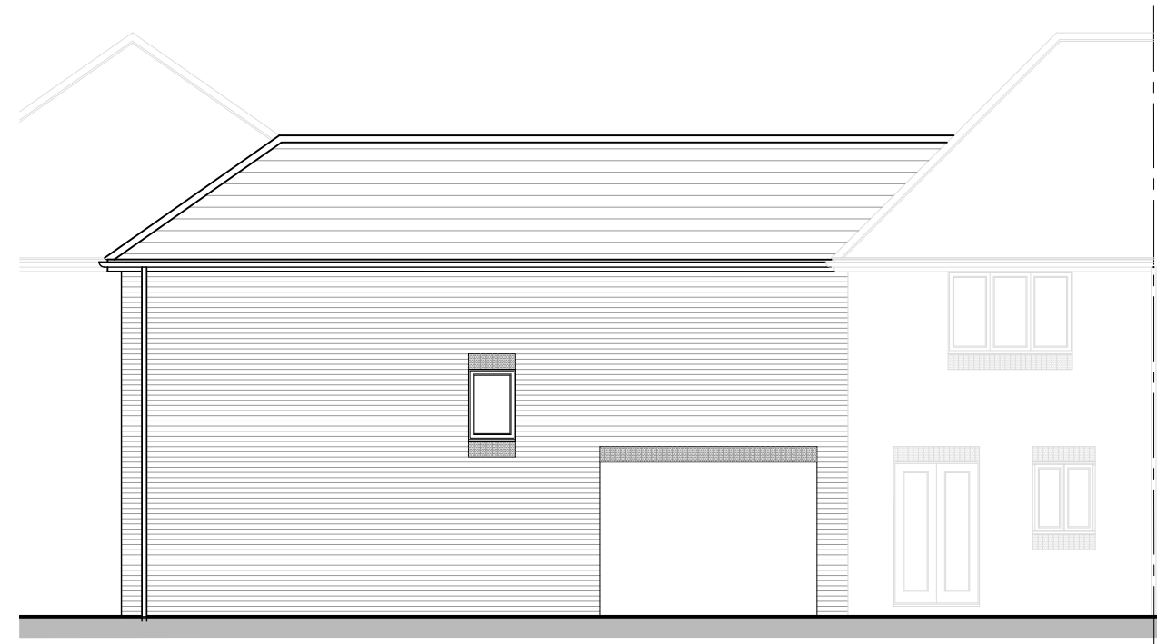
REAR ELEVATION
