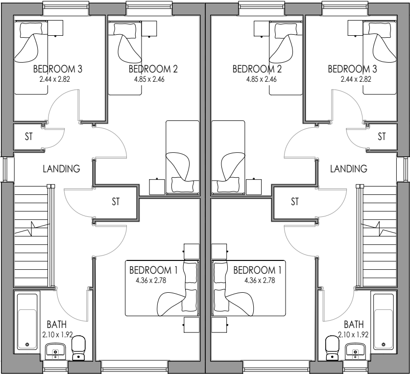
5P3B END AS FIRST FLOOR
