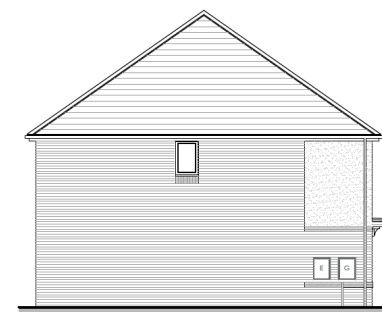
5P3B END AS SIDE ELEVATION
