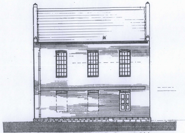
EASTERN (SIDE) ELEVATION EXISTING.
