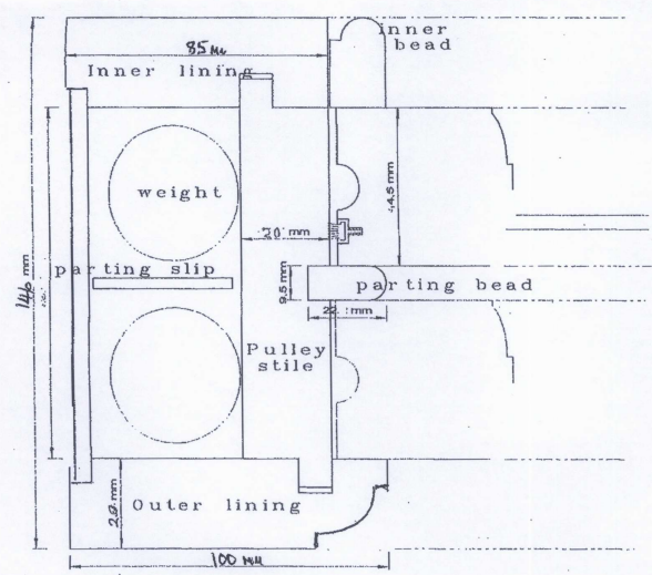
PLAN SECTION
