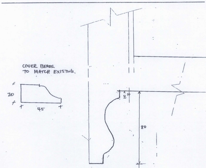
Sash horn detail TO MATCH EXISTING.
