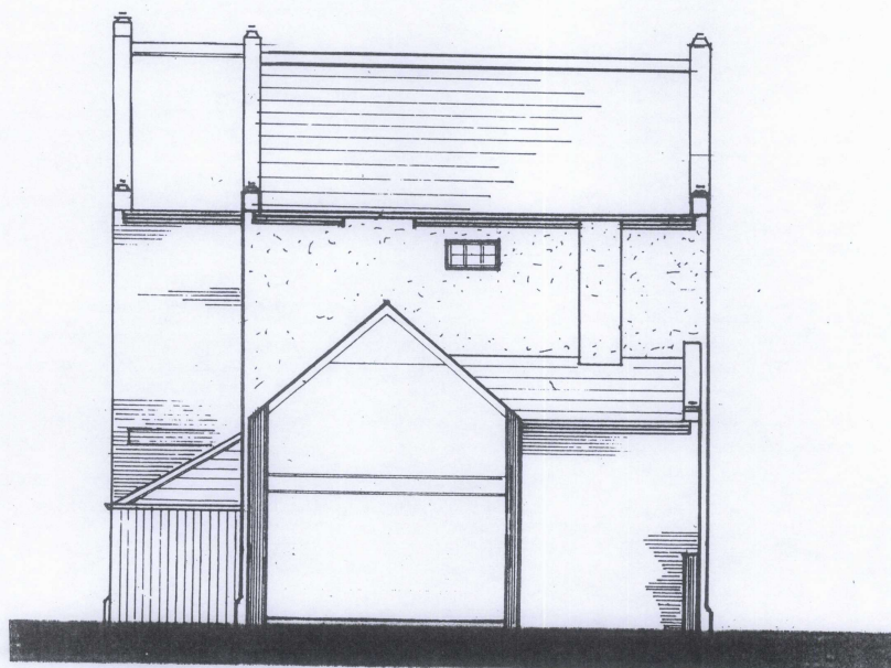
WESTERN (SIDE) ELEVATION PROPOSED.
