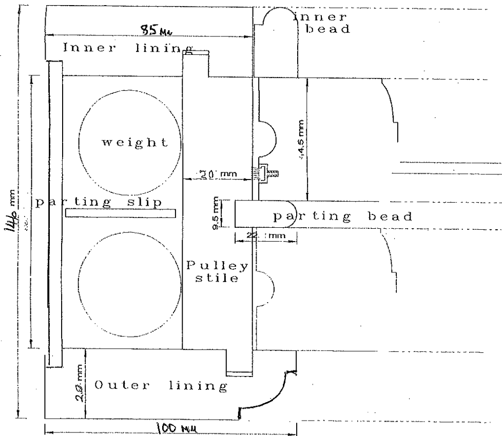
PLAN SECTION
