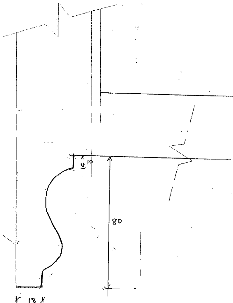
Sash horn detail TO MATCH EXISTING.
