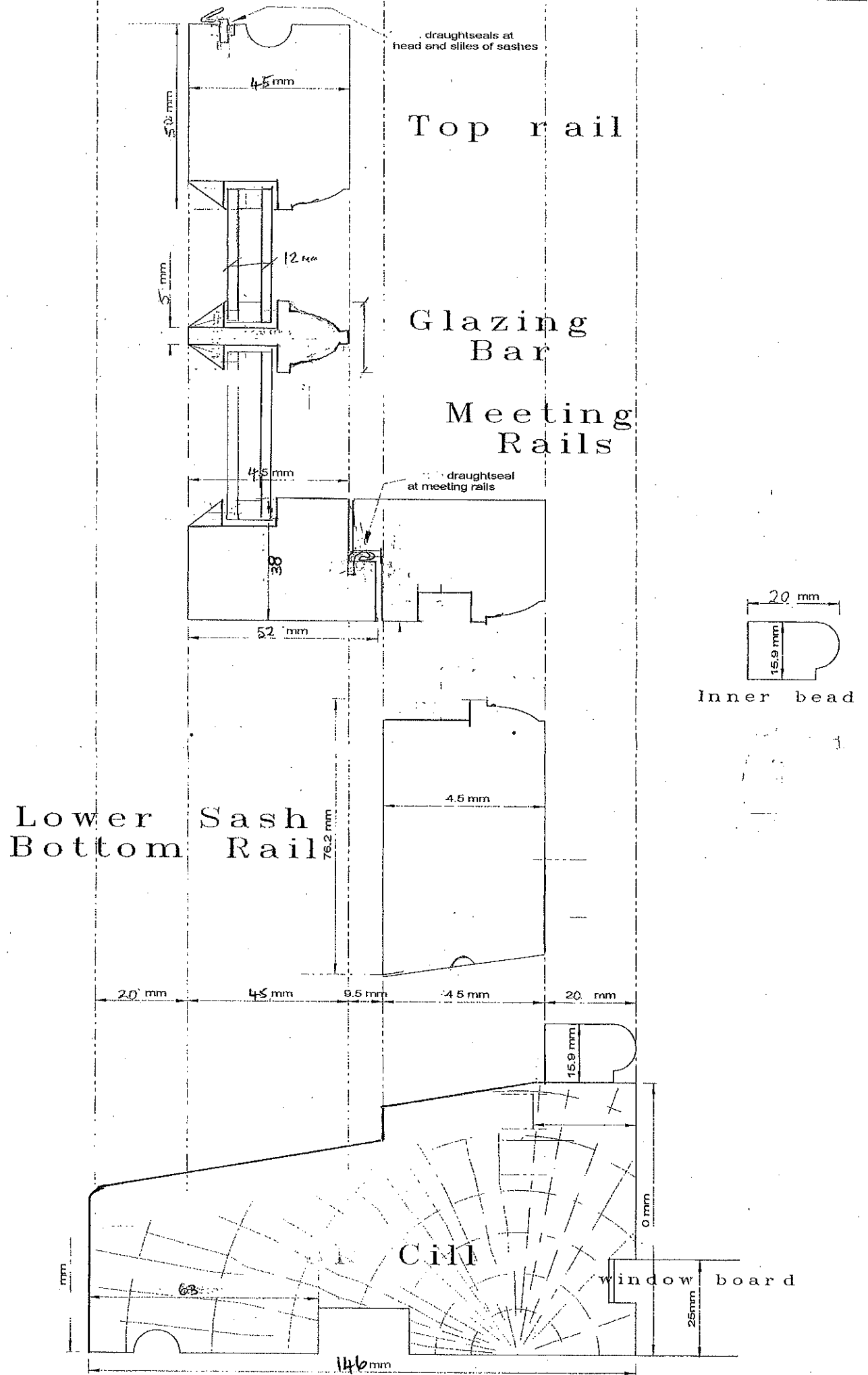
VERTICAL SECTION
