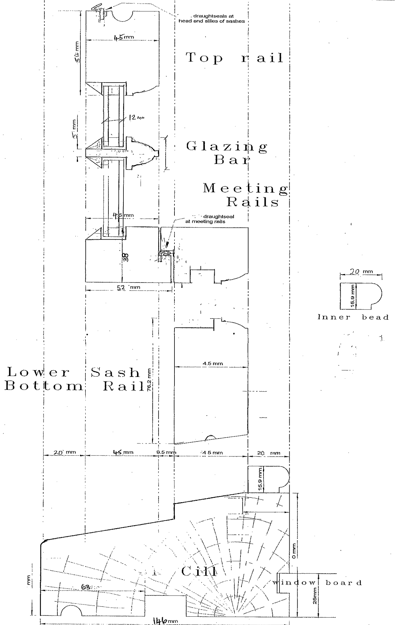
VERTICAL SECTION
