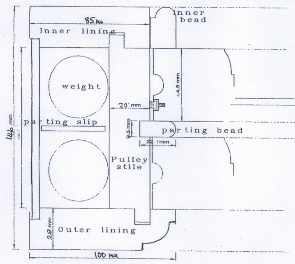
PLAN SECTION
