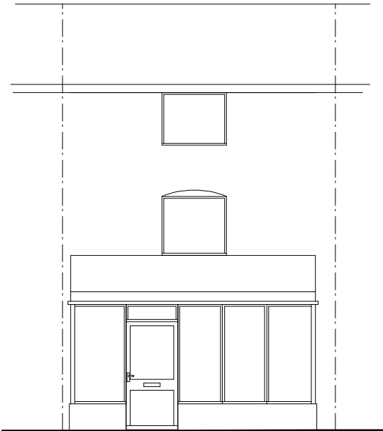
Front Elevation 1 : 100
