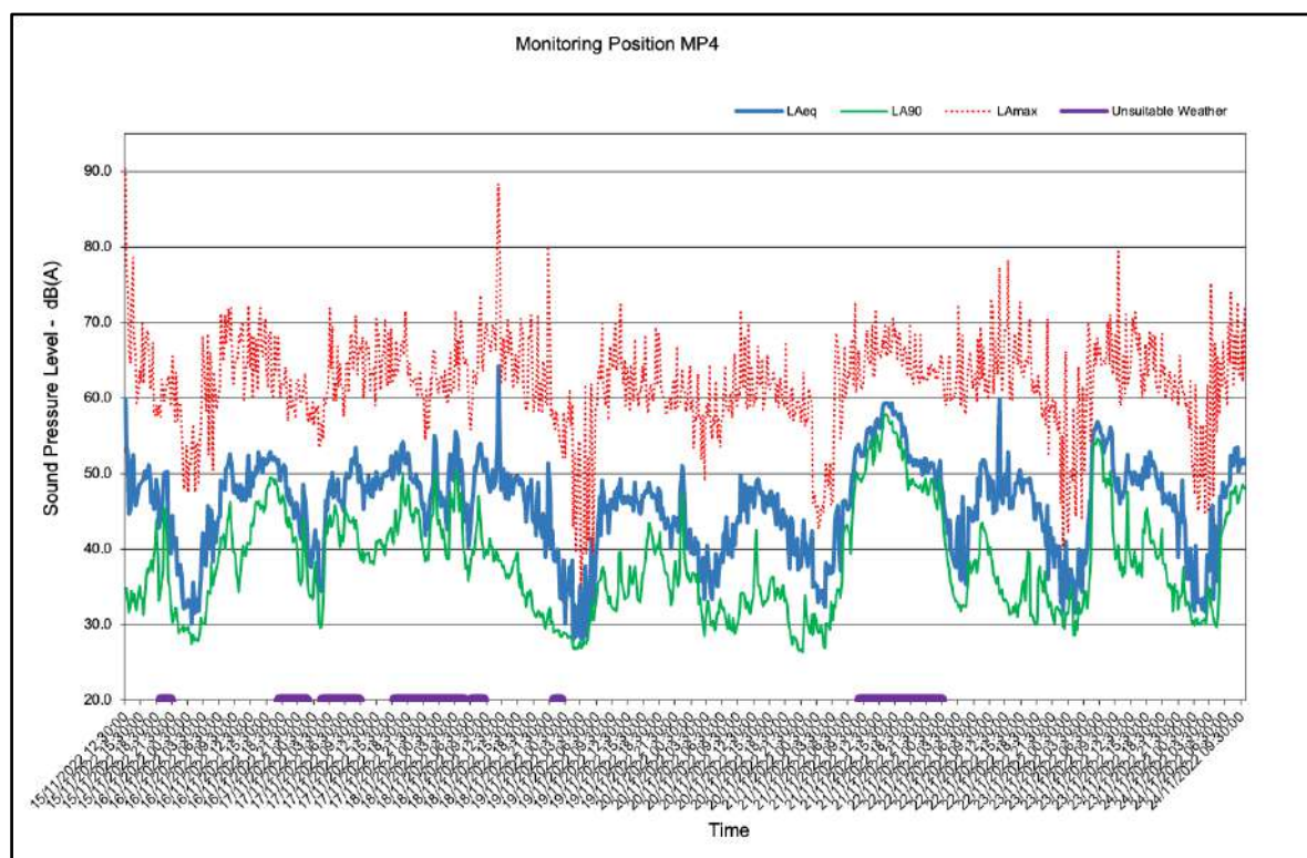
FIGURE 8: MEASURED TIME HISTORY – MP4
