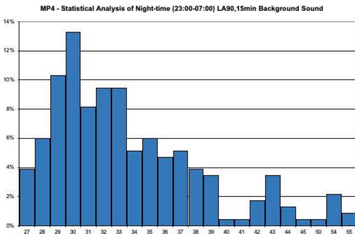
FIGURE 16: STATISTICAL ANALYSIS OF L_{A90} BACKGROUND – NIGHT-TIME – MP4
