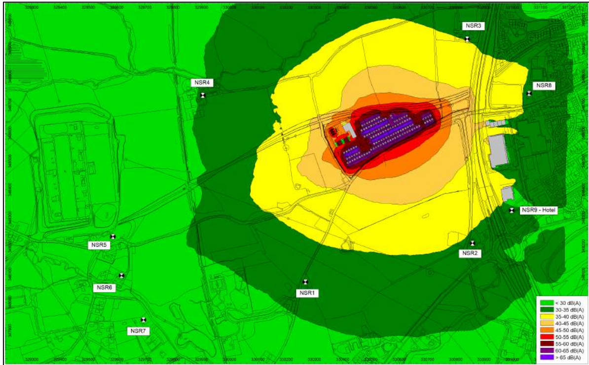
FIGURE 4: SPECIFIC SOUND LEVEL MAP
