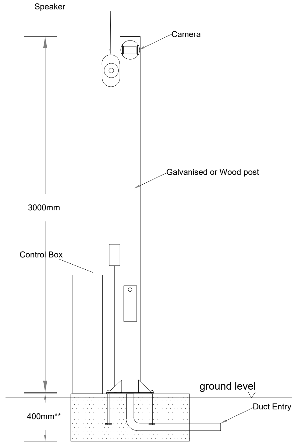
Side View
