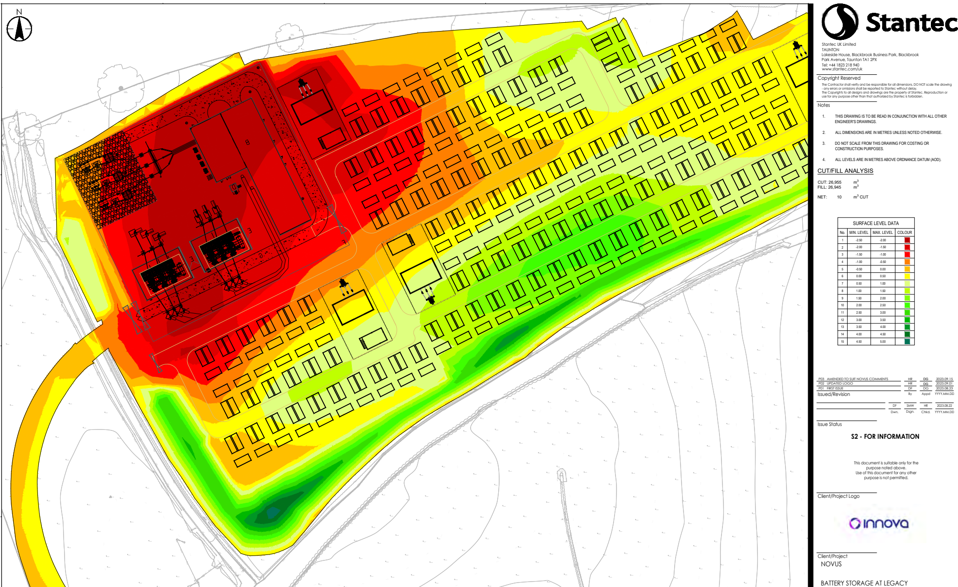
Figure 8. Extract of the Proposed Cut and Fill drawing prepared by Stantec.
