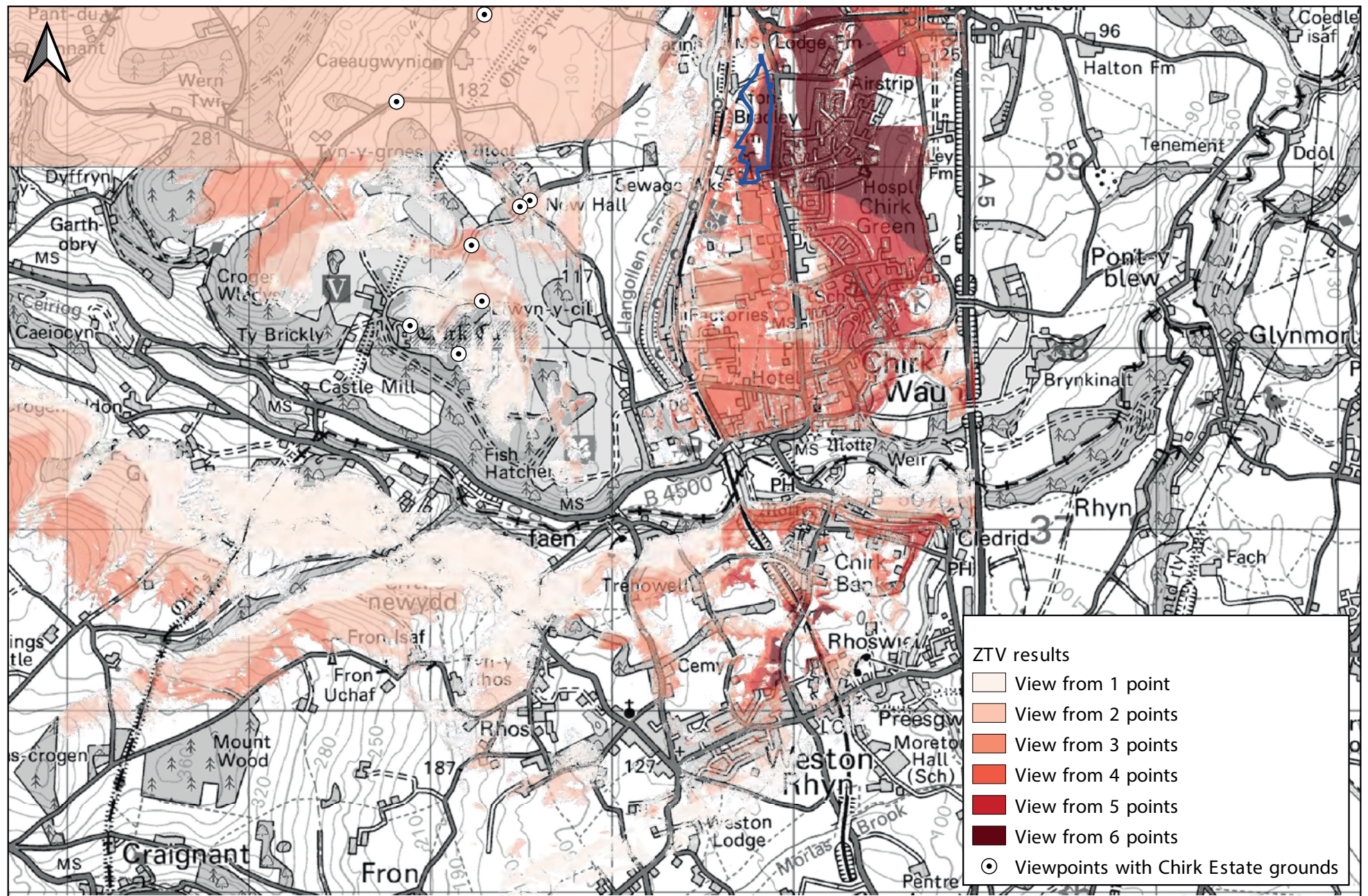
Figure 3. ZTV model produced from 6 points within the Registered Park and Garden of Chirk Castle.
