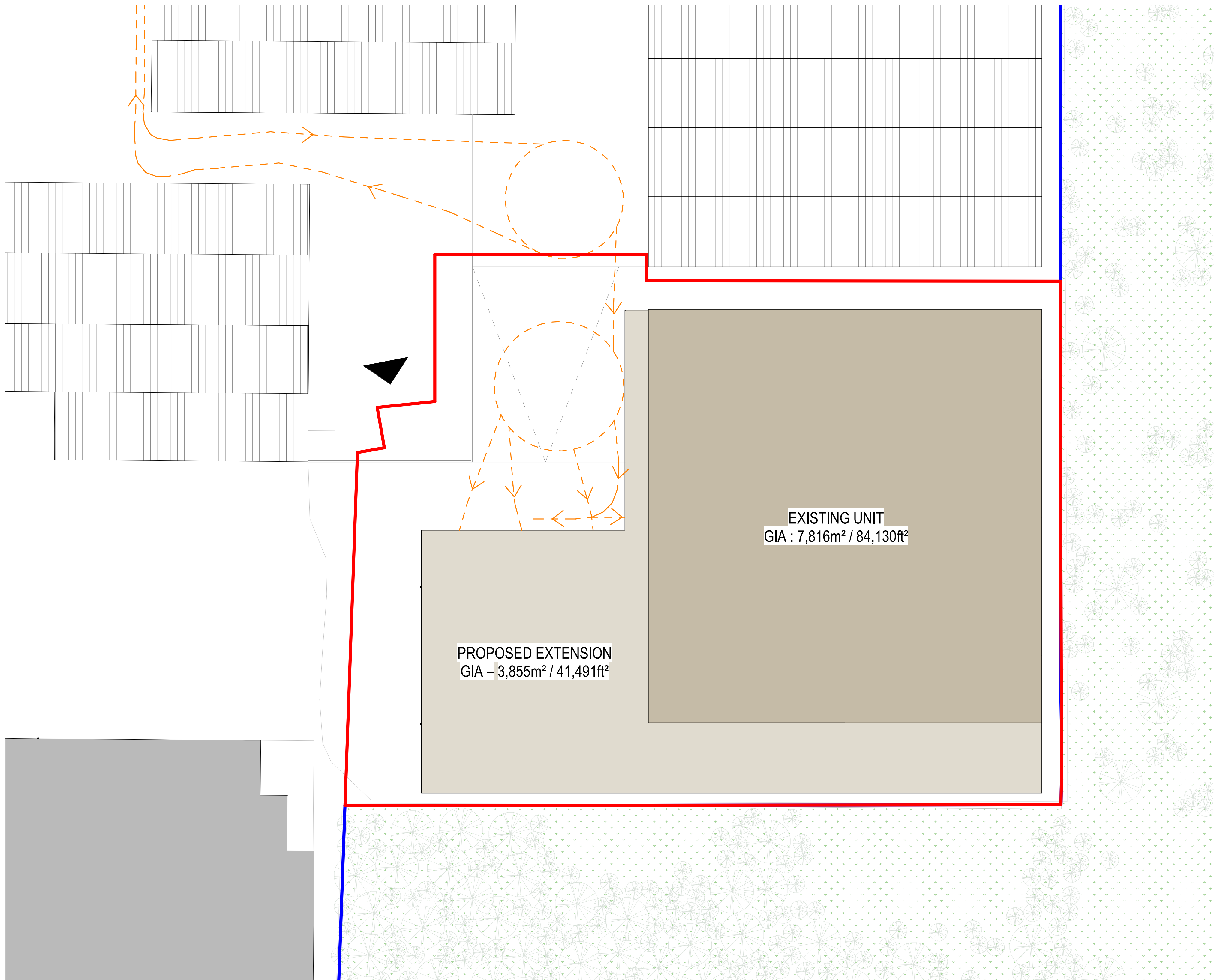
1 Proposed Access Plan Unit X 1 : 500
