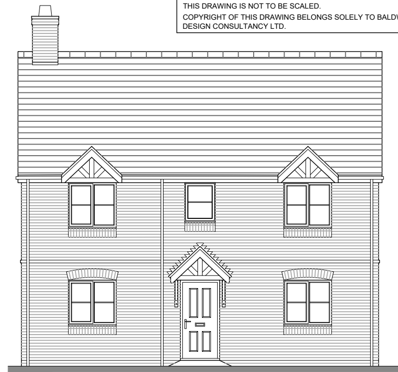
Front Elevation 'LANES' CHARACTER AREA
