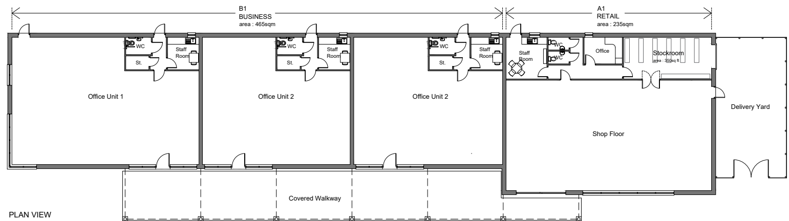
PLAN VIEW
