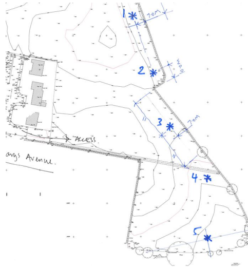
Site Layout
