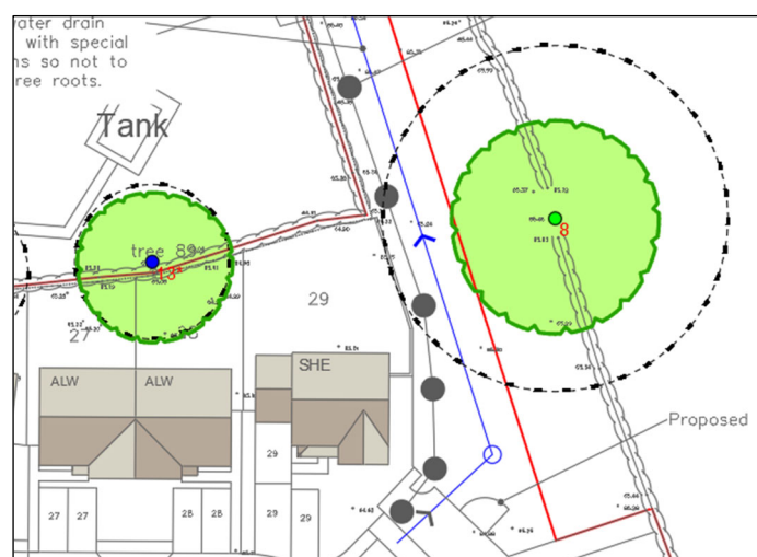
Plate 1 – original surface water drain alignment 10.8m from tree stem
