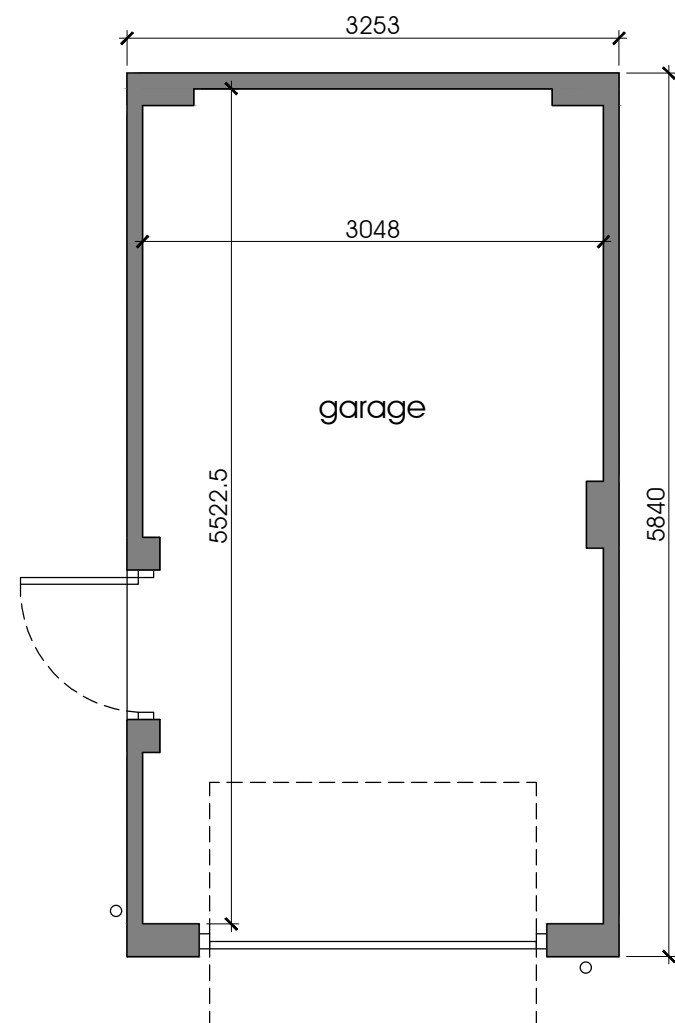
Floor Plan (1:50)
