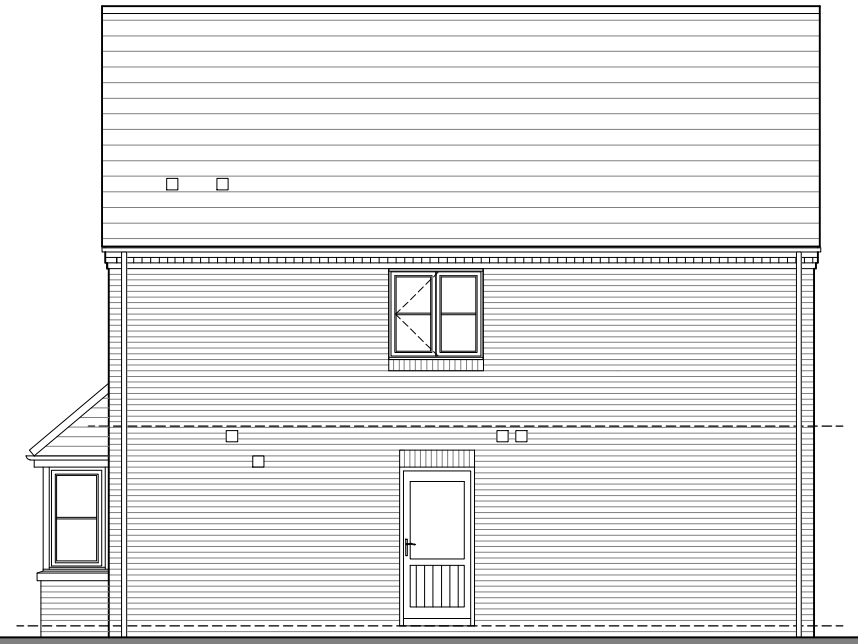
Rear Elevation
