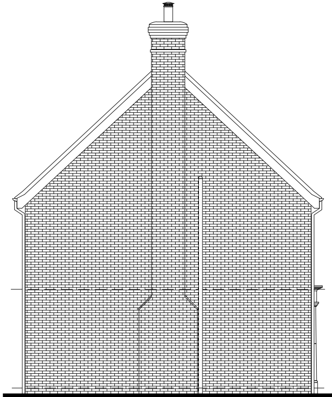
Side Elevation
