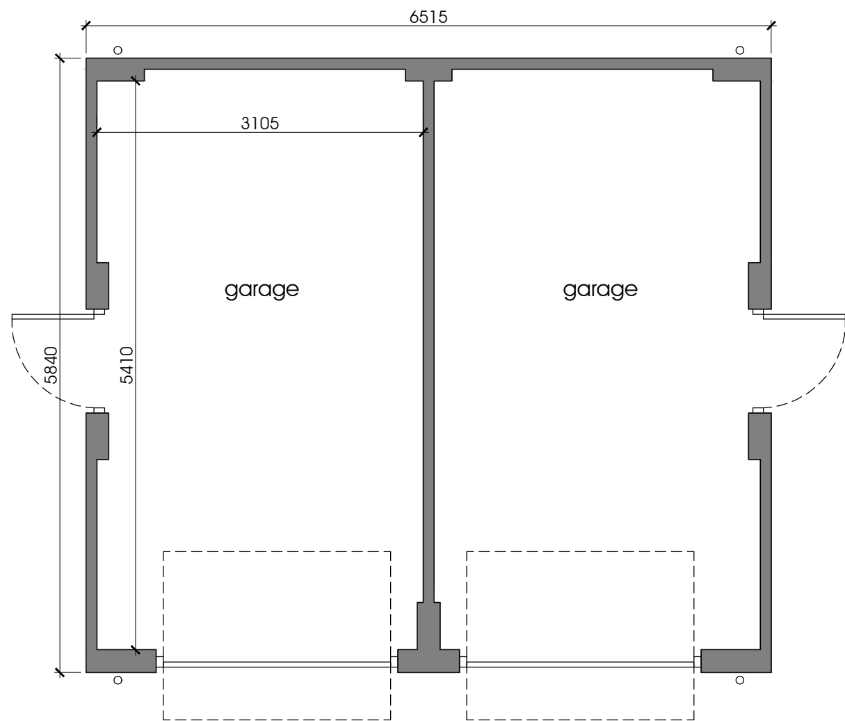
Floor Plan (1:50)
