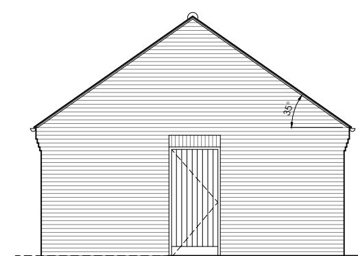
Elevations (1:100)
