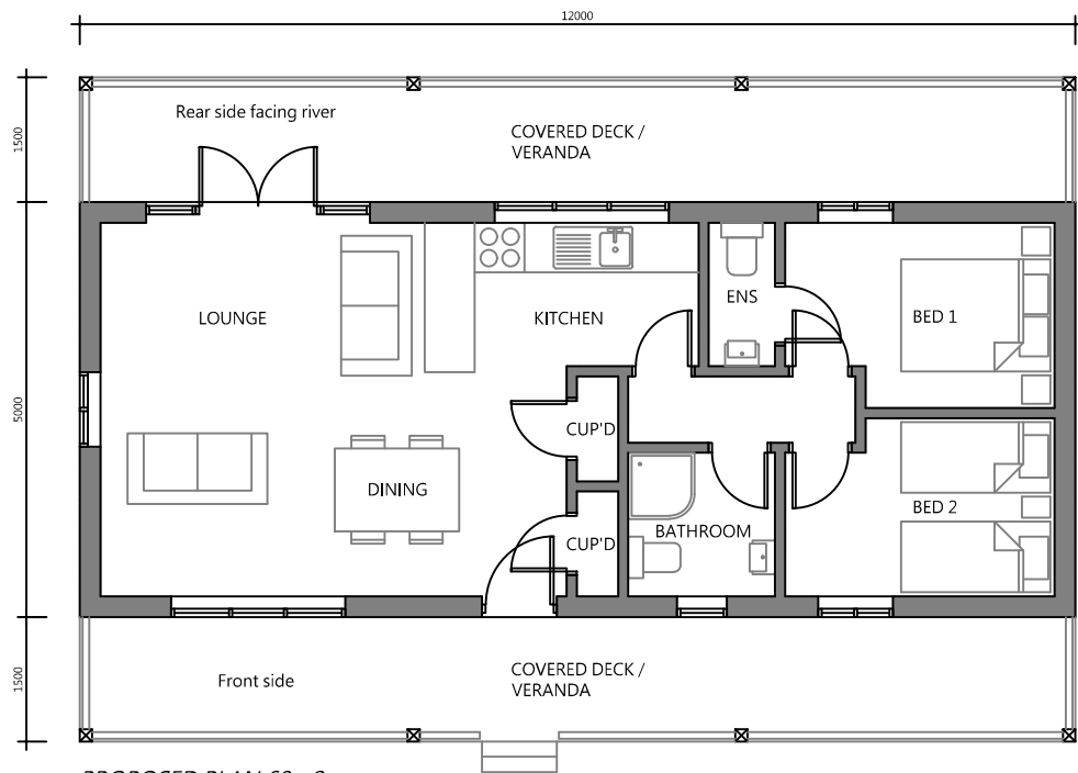
PROPOSED PLAN 60m2
