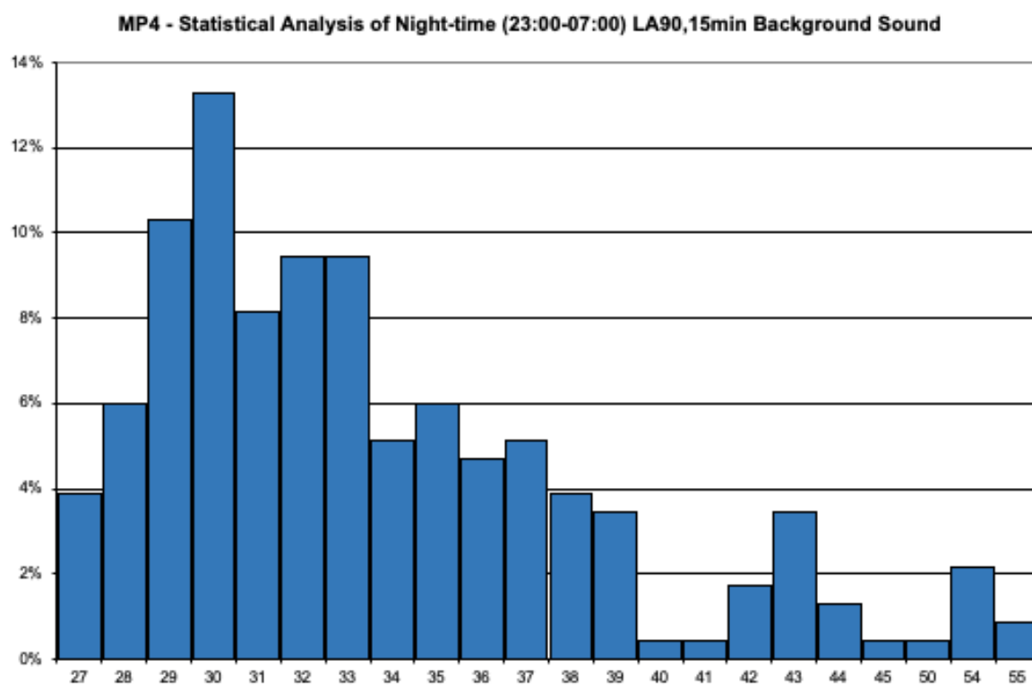
FIGURE 17: STATISTICAL ANALYSIS OF L_{A90} BACKGROUND – NIGHT-TIME – MP4
