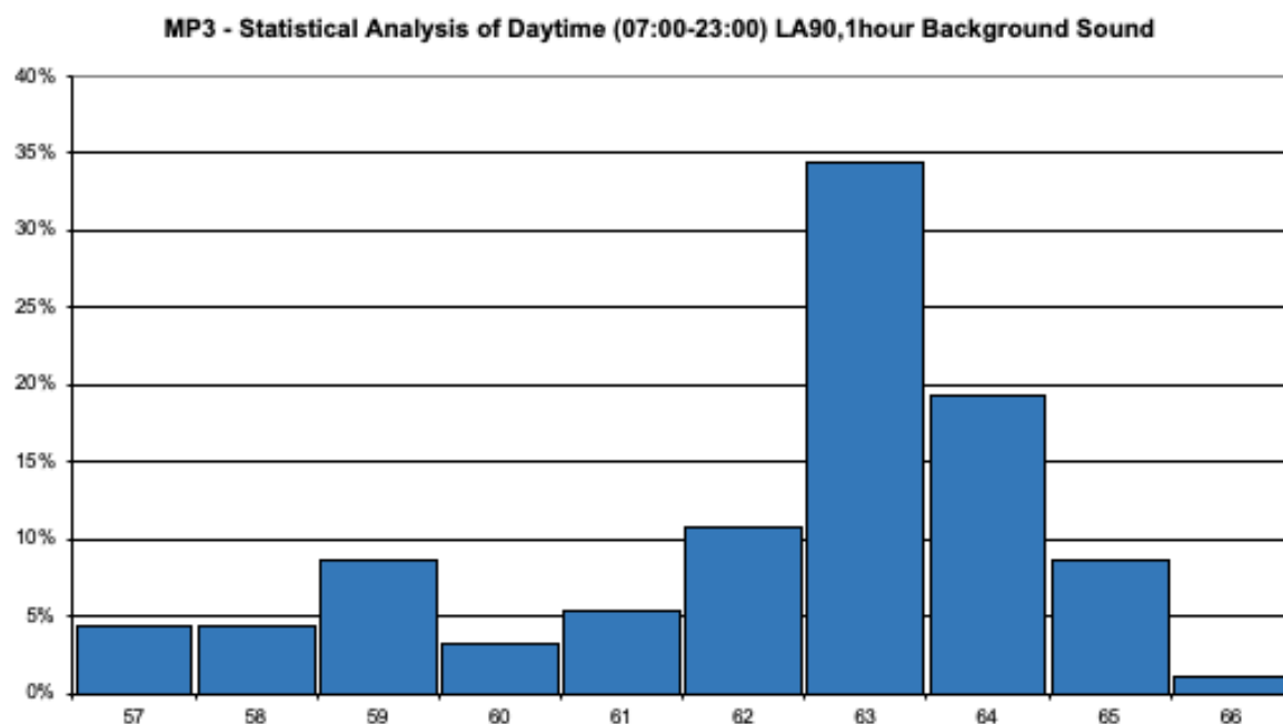
FIGURE 14: STATISTICAL ANALYSIS OF L_{A90} BACKGROUND – DAYTIME – MP3
