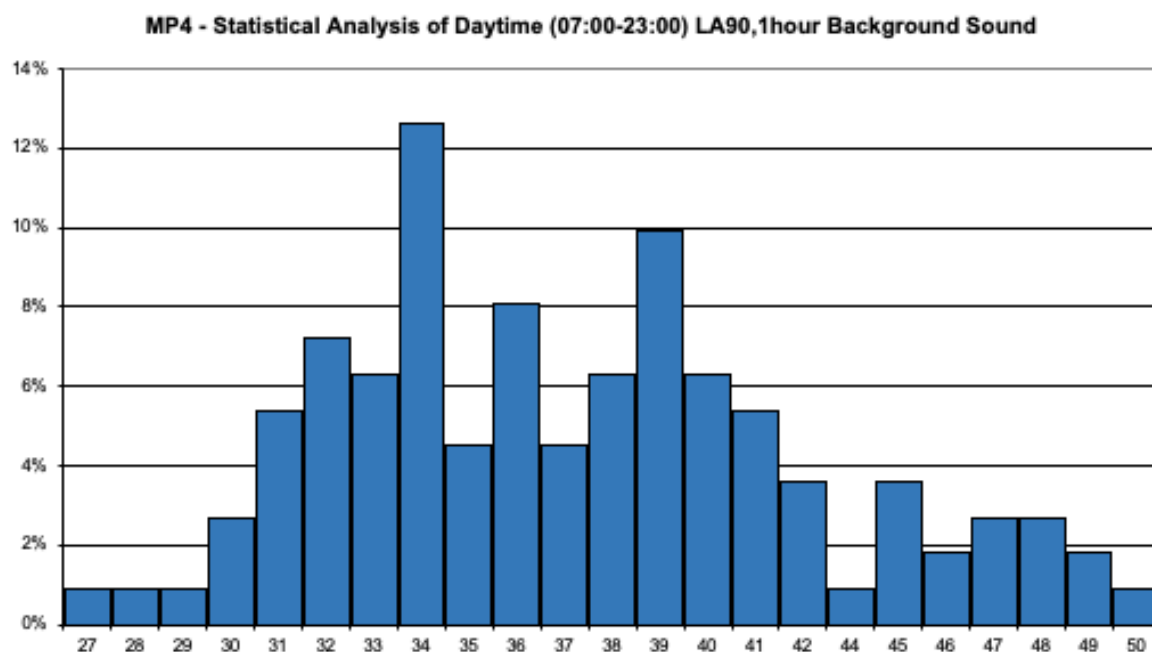
FIGURE 16: STATISTICAL ANALYSIS OF L_{A90} BACKGROUND – DAYTIME – MP4
