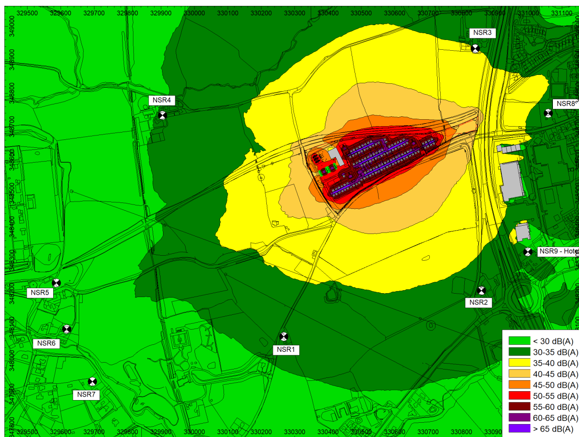
FIGURE 5: SPECIFIC SOUND LEVEL MAP – NIGHT-TIME
