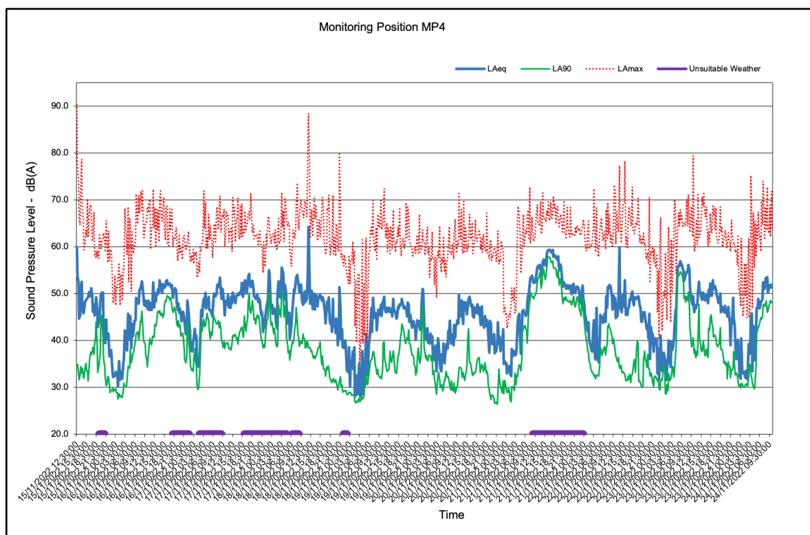
FIGURE 9: MEASURED TIME HISTORY – MP4
