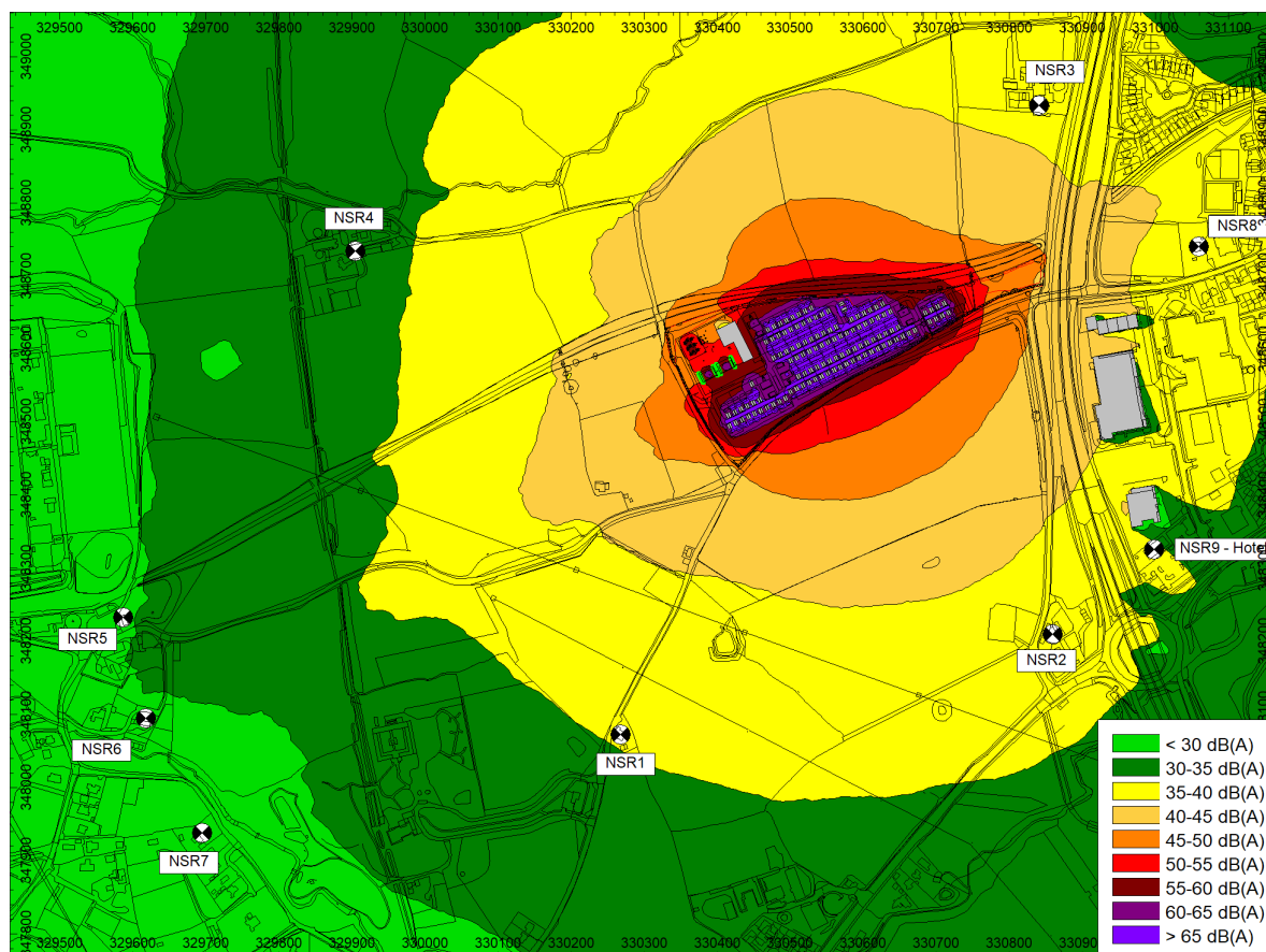
FIGURE 4: SPECIFIC SOUND LEVEL MAP - DAYTIME
