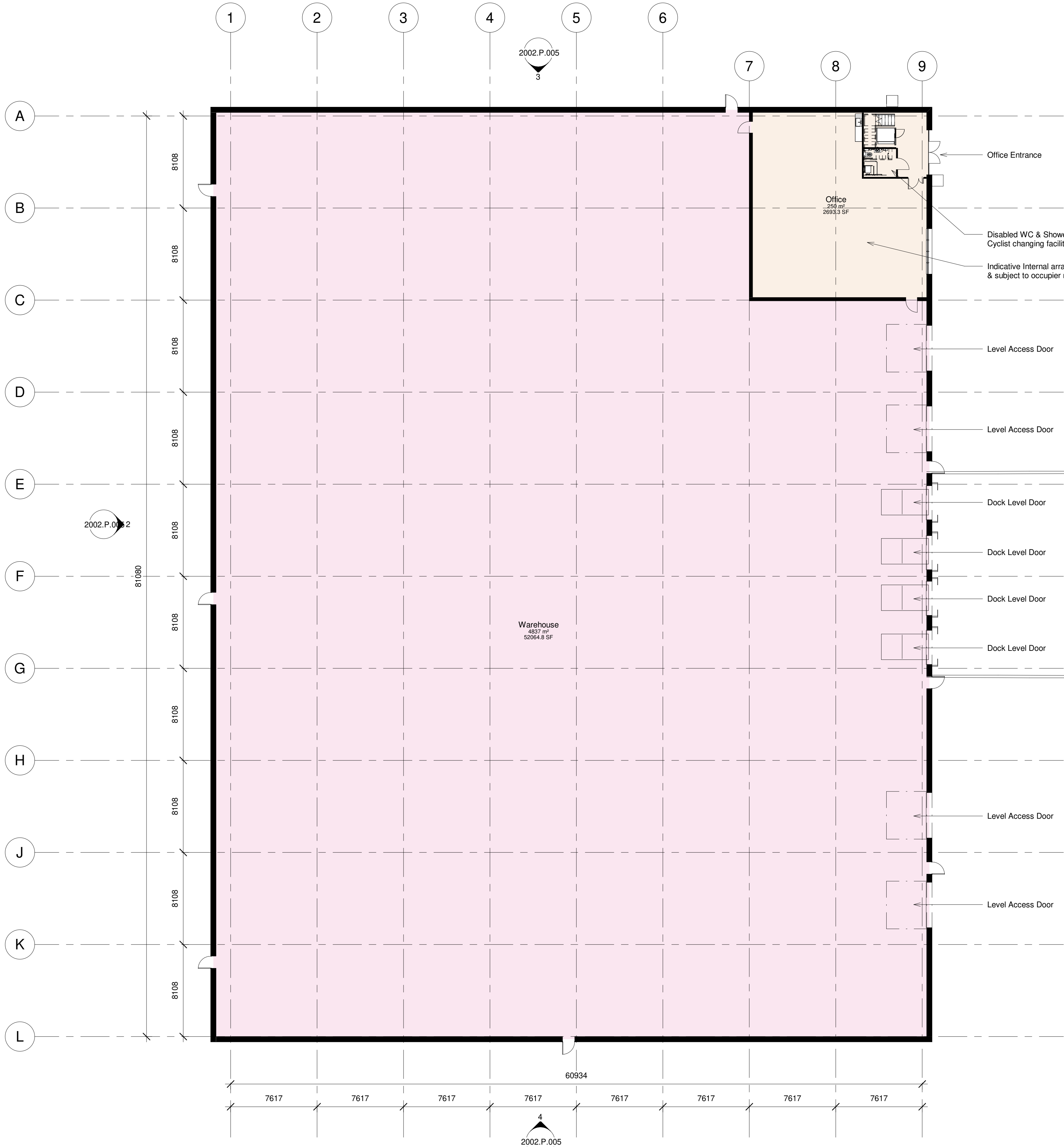
1 GROUND FLOOR 1 : 200
