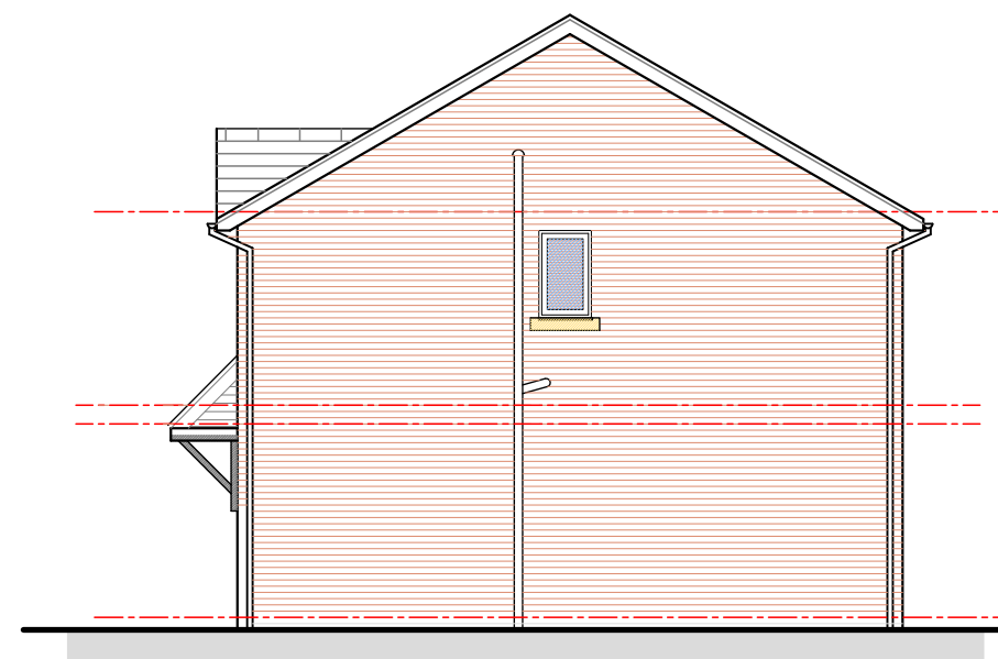
Plot 1 Side Elevation
