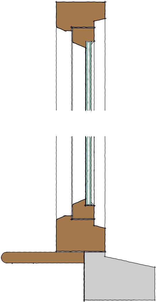
TYPICAL SECTIONS SCALE 1.5
