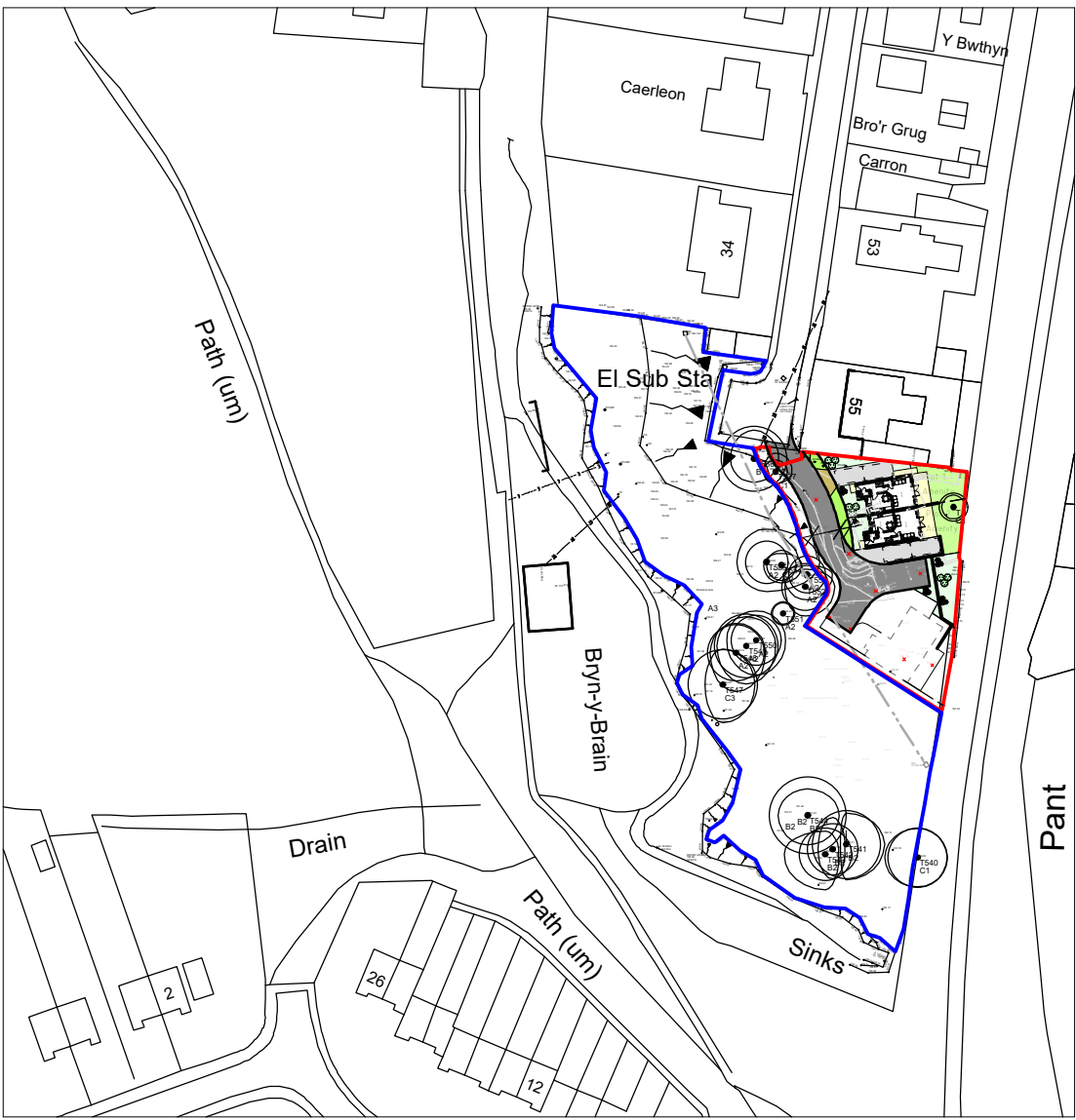
Location Plan 1:1250
