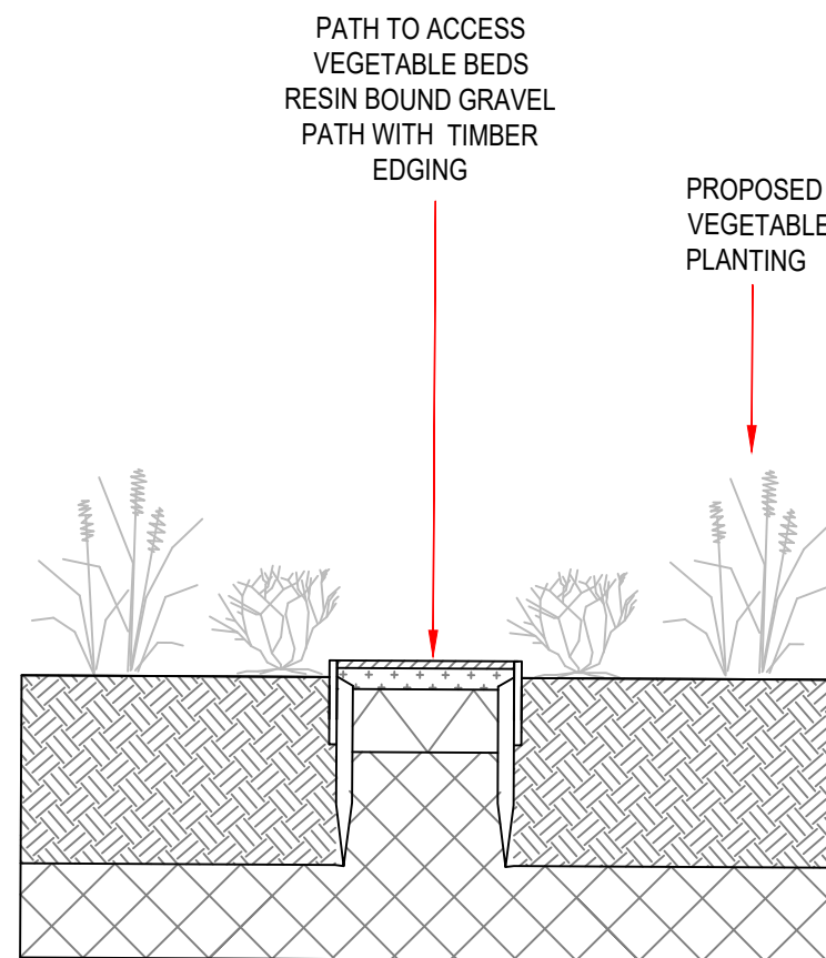
7 1:20 ANDERSON SHELTER - ACCESS PATH TO VEGETABLE BEDS
