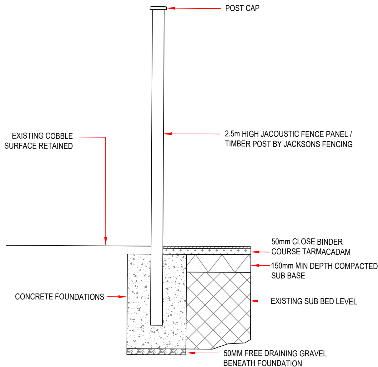
6 1:20 CLOSE BOARD TIMBER SECURITY FENCE
