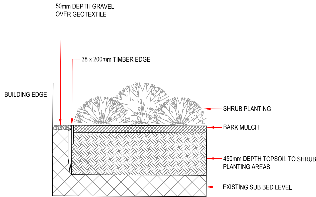
1 1:20 GRAVEL EDGE TO PLANTING BED / BUILDING INTERFACE
