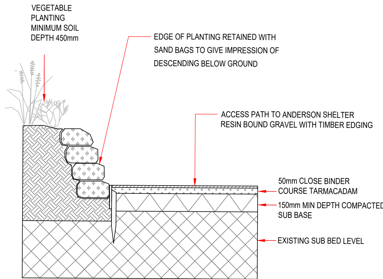
8 1:20 ACCESS PATH INTO ANDERSON SHELTER
