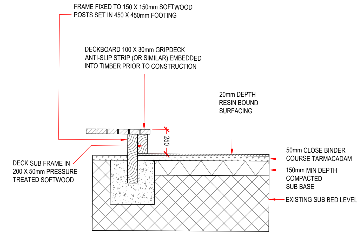
3 1:20 STAGE - TIMBER DECKED STRUCTURE
