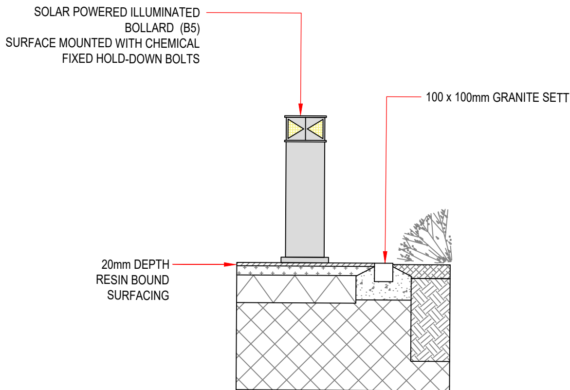
4 1:20 BOLLARD SET IN HARD LANDSCAPE
