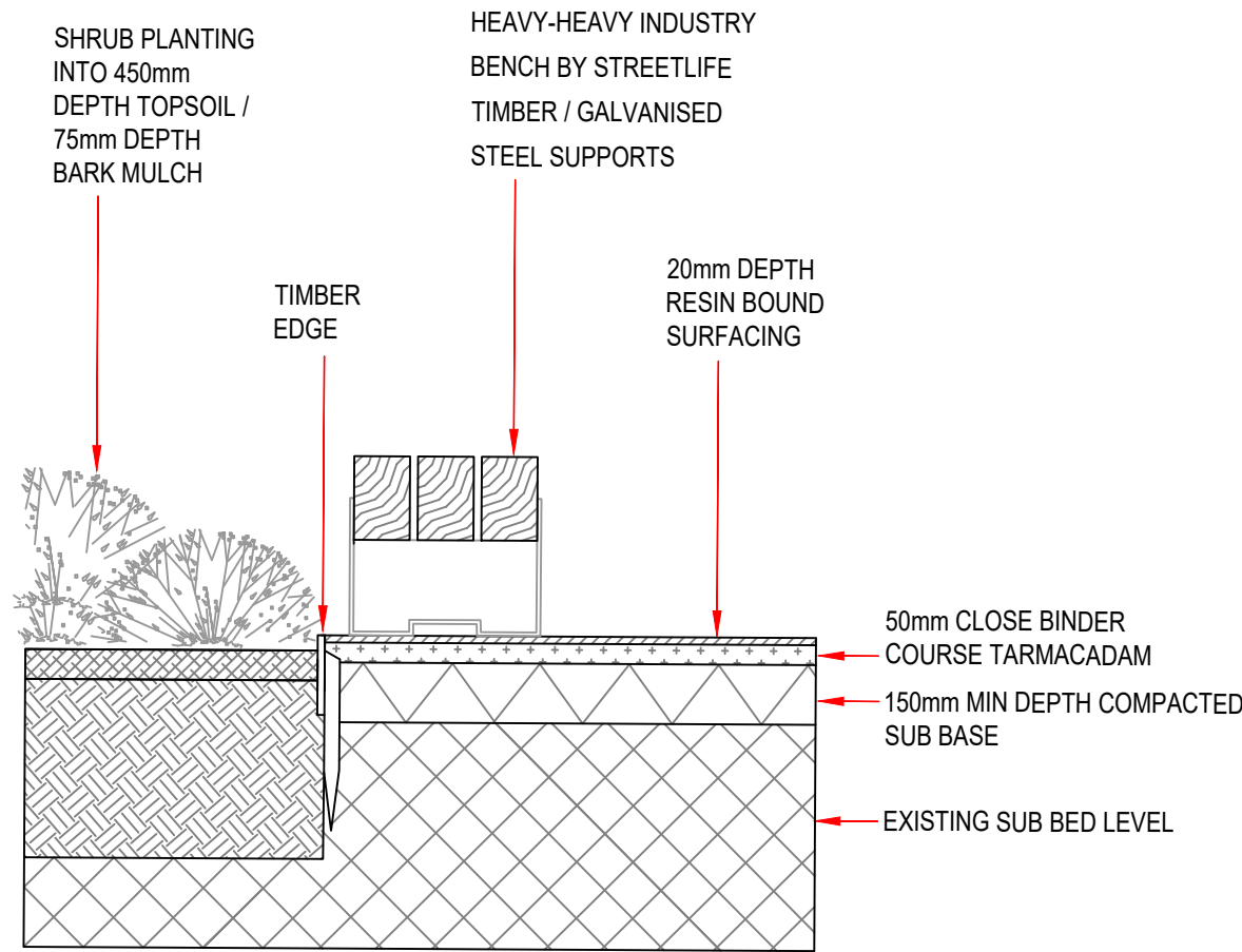
2 1:20 TIMBER BENCH ADJACENT TO PLANTING AREA / STAGE
